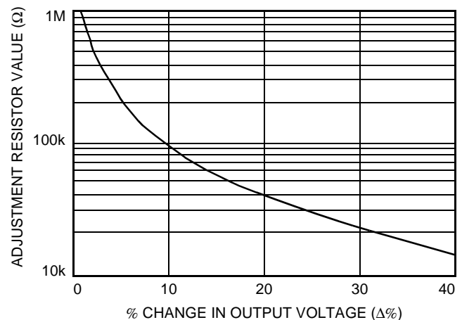
Figure 22. Resistor Selection for Decreased Output Voltage
