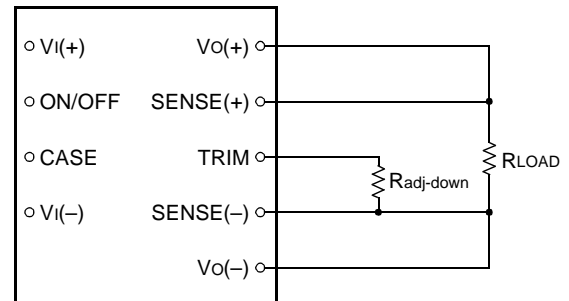
Figure 21. Circuit Configuration to Decrease Output Voltage
