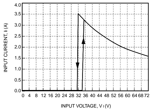
Figure 3. Typical JFW100H Input Characteristics at Room Temperature, I_o = I_{o, \max}
