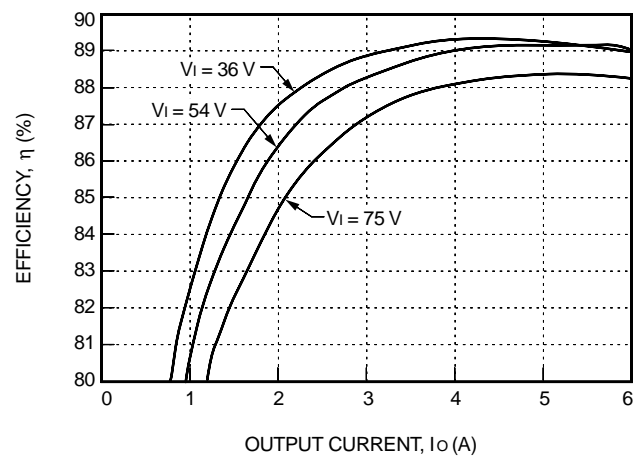
Figure 12. Typical JFW150H Converter Efficiency vs. Output Current at Room Temperature
