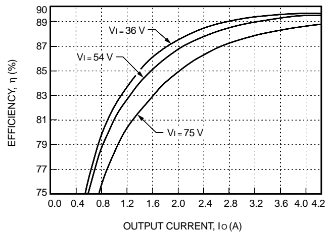
Figure 11. Typical JFW100H Converter Efficiency vs. Output Current at Room Temperature
