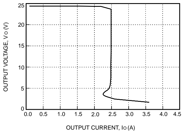
Figure 5. Typical JFW050H Output Characteristics at Room Temperature, V_i = 48 V
