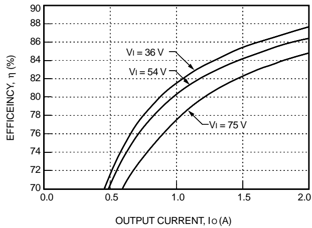
Figure 9. Typical JFW050H Converter Efficiency vs. Output Current at Room Temperature
