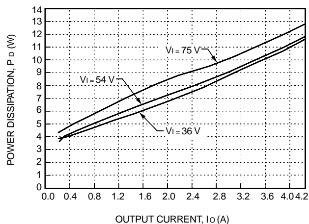
Figure 31. JFW100H Power Dissipation vs. Output Current at 25 °C
