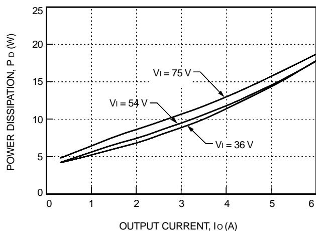
Figure 32. JFW150H Power Dissipation vs. Output Current at 25 °C
