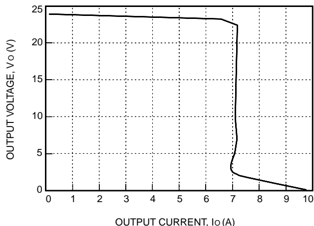
Figure 8. Typical JFW150H Output Characteristics at Room Temperature, V_i = 48 V
