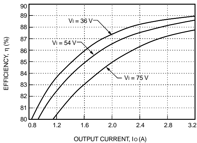
Figure 10. Typical JFW075H Converter Efficiency vs. Output Current at Room Temperature
