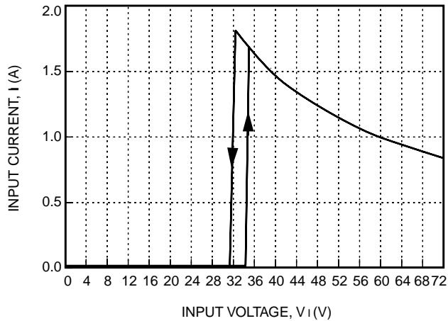
Figure 1. Typical JFW050H Input Characteristics at Room Temperature, I_o = I_{o, \max}
