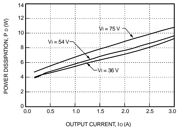
Figure 30. JFW075H Power Dissipation vs. Output Current at 25 °C
