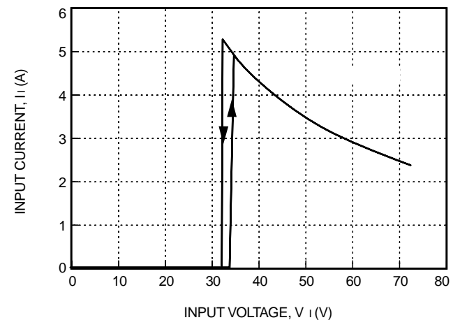
Figure 4. Typical JFW150H Input Characteristics at Room Temperature, I_o = I_{o, \max}
