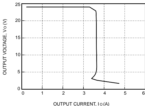
Figure 6. Typical JFW075H Output Characteristics at Room Temperature, V_i = 48 V
