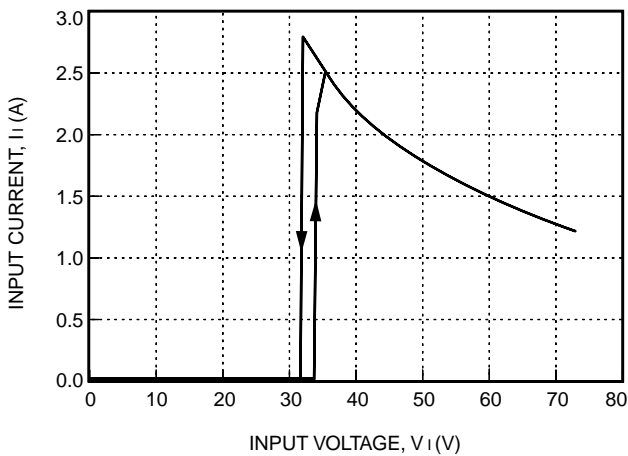
Figure 2. Typical JFW075H Input Characteristics at Room Temperature, I_o = I_{o, \max}
