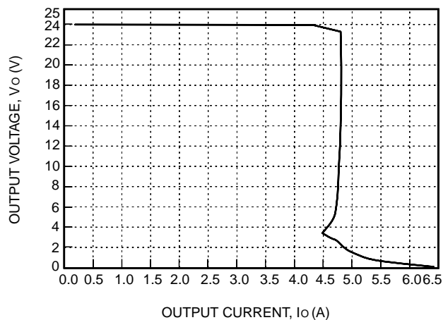
Figure 7. Typical JFW100H Output Characteristics at Room Temperature, V_i = 48 V
