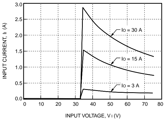
Figure 2. Typical JFW150G Input Characteristics at Room Temperature
