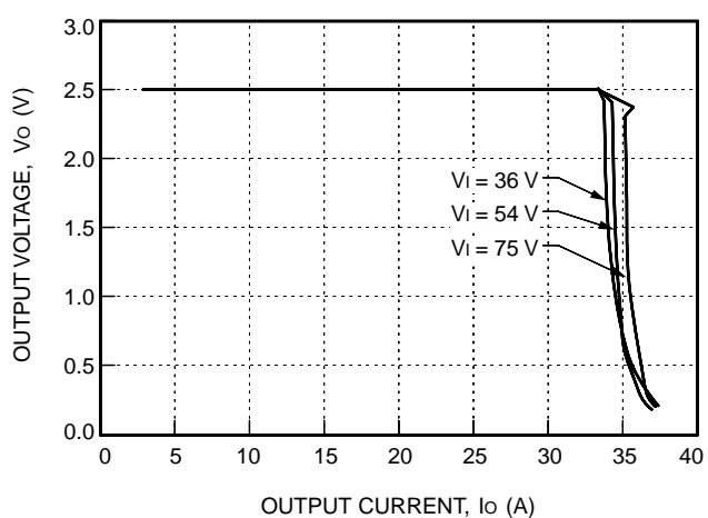
Figure 4. Typical JFW150G Output Characteristics at Room Temperature
