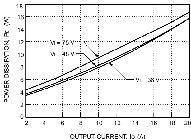
Figure 23. JFW100G Power Dissipation vs. Output Current at 80 °C
