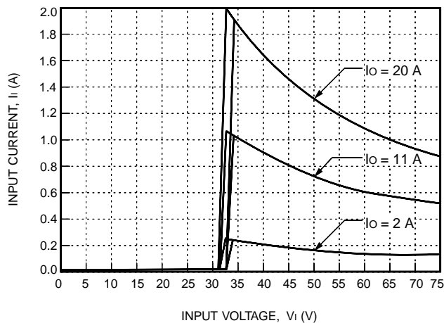
Figure 1. Typical JFW100G Input Characteristics at Room Temperature
