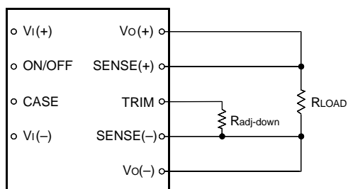
Figure 16. Circuit Configuration to Decrease Output Voltage
