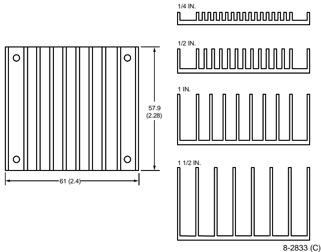
Figure 28. Transverse Heat Sink
