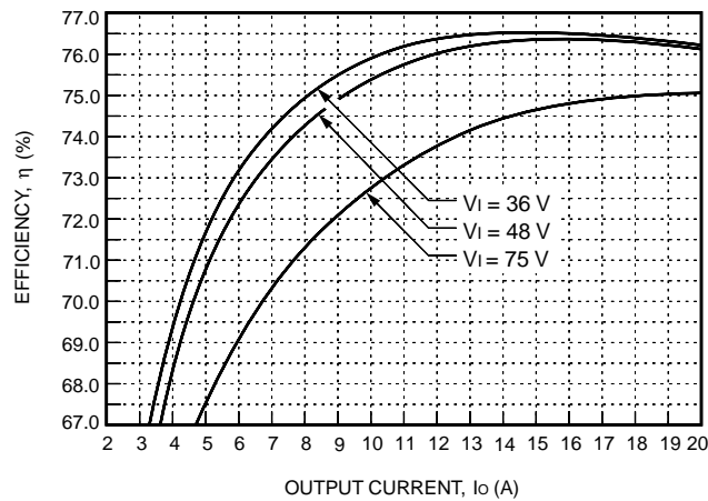
Figure 5. Typical JFW100G Converter Efficiency vs. Output Current at Room Temperature
