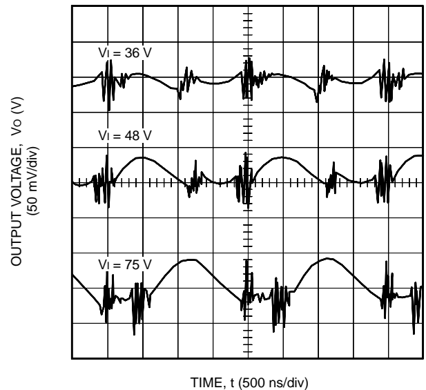
Figure 7. Typical JFW150G Output Ripple Voltage at Room Temperature, and I_o = I_{o, max}
