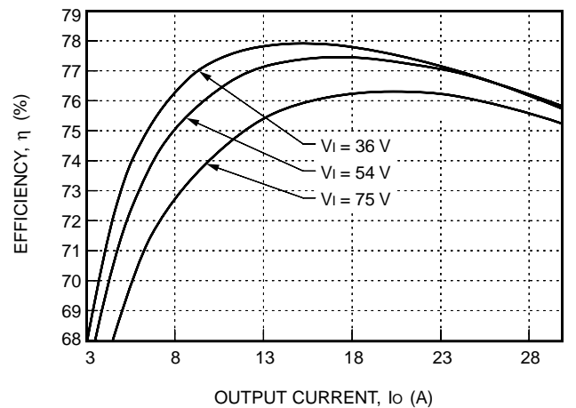
Figure 6. Typical JFW150G Converter Efficiency vs. Output Current at Room Temperature
