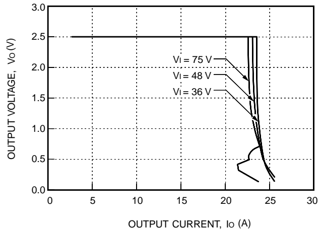
Figure 3. Typical JFW100G Output Characteristics at Room Temperature
