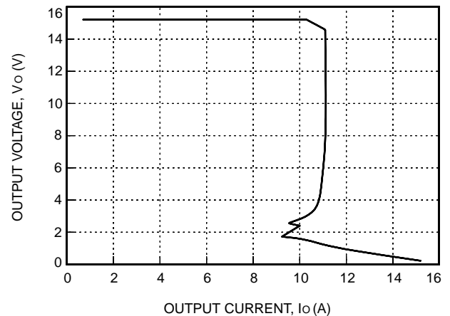
Figure 8. Typical JFW150C Output Characteristics at Room Temperature, V_I = 48 V
