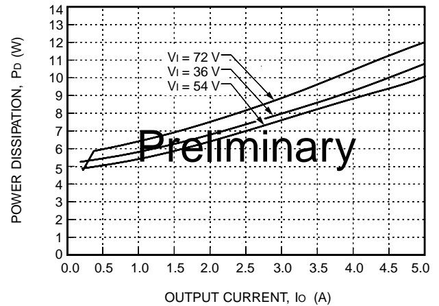
Figure 30. JFW075C Power Dissipation vs. Output Current
