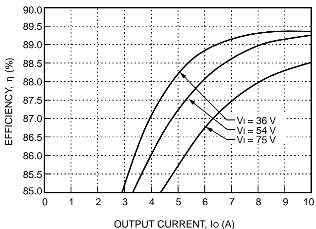
Figure 12. Typical JFW150C Converter Efficiency vs. Output Current at Room Temperature
