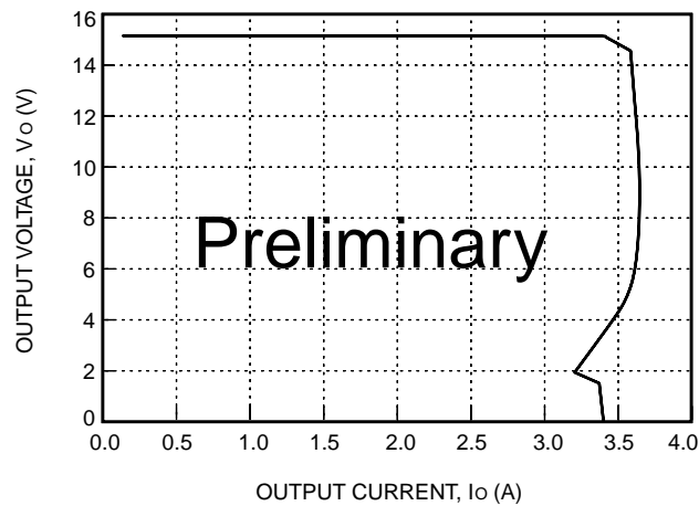
Figure 5. Typical JFW050C Output Characteristics at Room Temperature, V_I = 48 V
