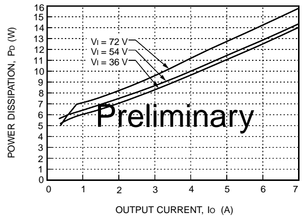
Figure 31. JFW100C Power Dissipation vs. Output Current
