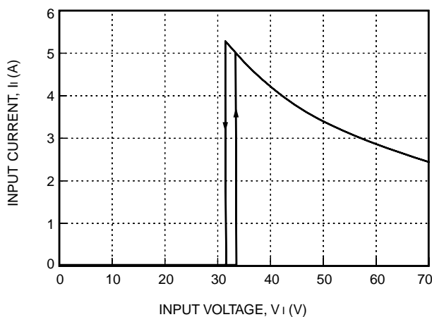
Figure 4. Typical JFW150C Input Characteristics at Room Temperature, I_o = I_{o, max}
