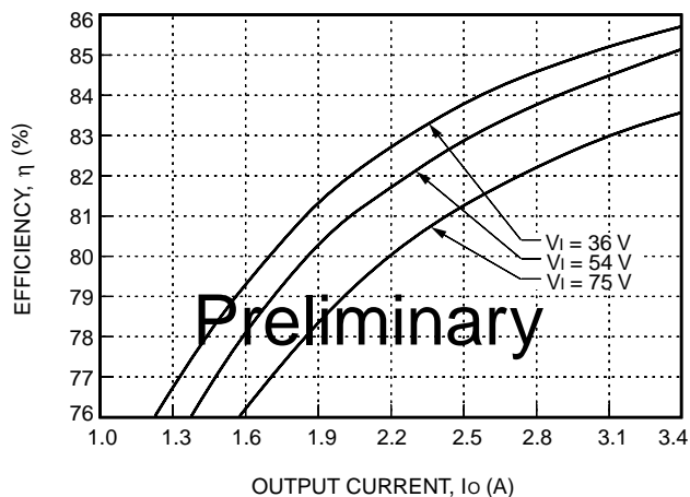
Figure 9. Typical JFW050C Converter Efficiency vs. Output Current at Room Temperature
