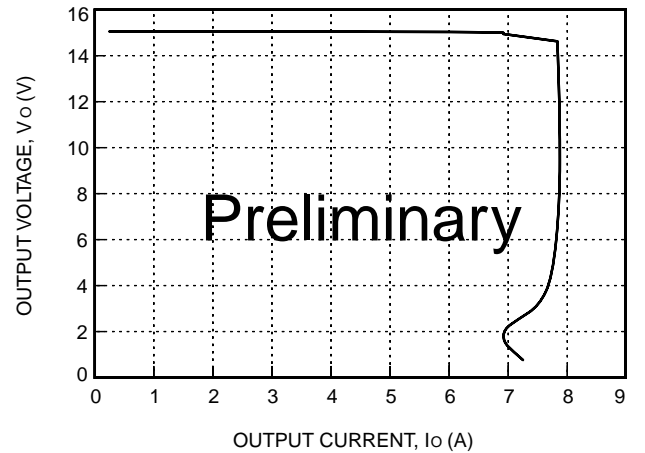
Figure 7. Typical JFW100C Output Characteristics at Room Temperature, V_I = 48 V
