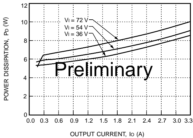
Figure 29. JFW050C Power Dissipation vs. Output Current
