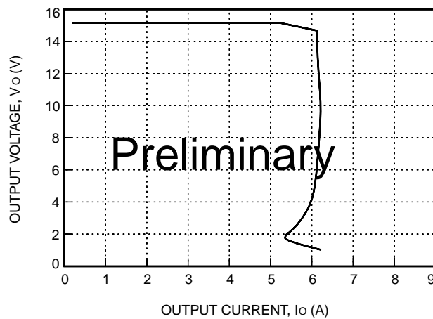
Figure 6. Typical JFW075C Output Characteristics at Room Temperature, V_I = 48 V
