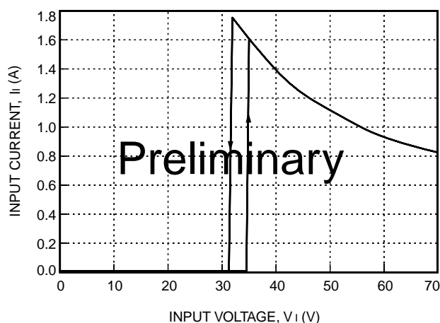
Figure 1. Typical JFW050C Input Characteristics at Room Temperature, I_o = I_{o, max}
