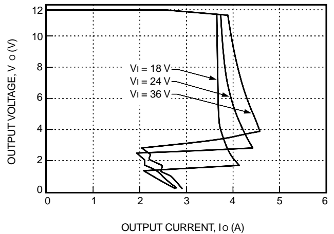
Figure 8. JC030B-M Typical Output Characteristics
