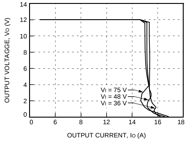
Figure 8. Typical JFW150B Output Characteristics at Room Temperature
