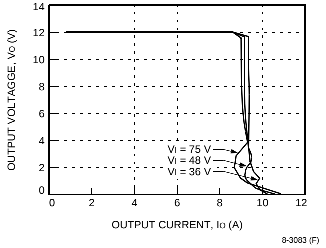
Figure 7. Typical JFW100B Output Characteristics at Room Temperature
