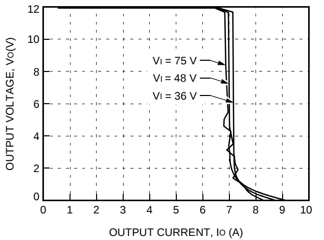
Figure 6. Typical JFW075B Output Characteristics at Room Temperature
