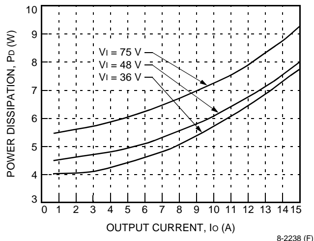
Figure 23. JAHW075A Power Dissipation vs. Output Current at 25 °C
