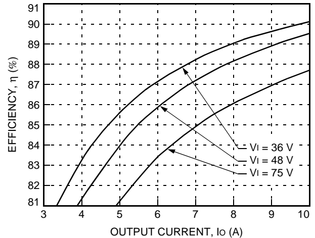
Figure 3. Typical JAHW050A Converter Efficiency vs. Output Current at Room Temperature
