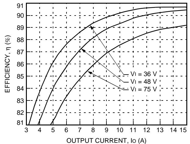
Figure 4. Typical JAHW075A Converter Efficiency vs. Output Current at Room Temperature
