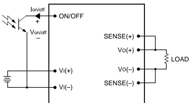
Figure 15. Remote On/Off Implementation Tyco Electronics Corp.
