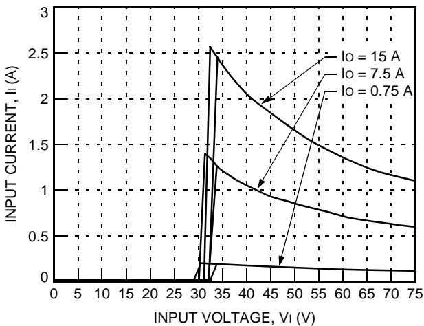
Figure 2. Typical JAHW075A Input Characteristics at Room Temperature
