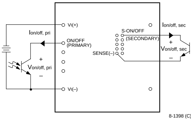
Figure 11. Remote On/Off Implementation
