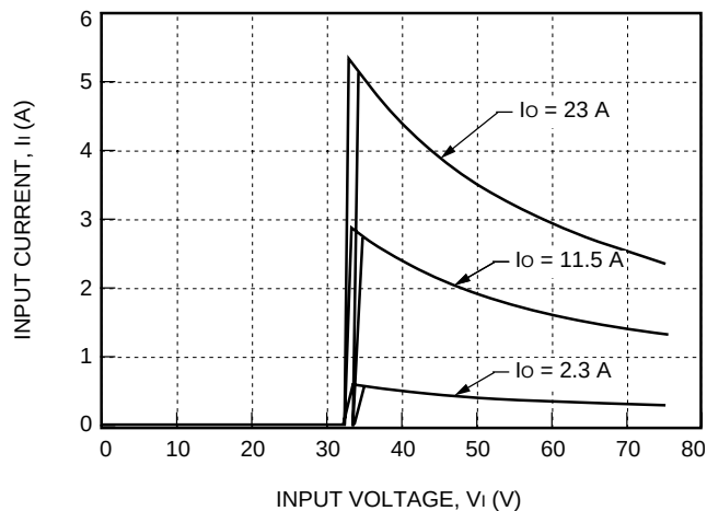
Figure 1. Typical JFW150S6R5 Input Characteristics at Room Temperature
