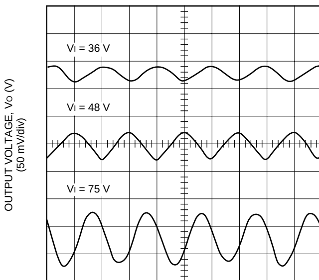
Figure 4. Typical JFW150S6R5 Output Ripple Voltage at Room Temperature, I_o = I_{o, \max}
