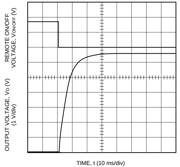
Figure 7. Typical Start-Up from Remote On/Off JFW150S6R51; I_o = I_{o, \max}
