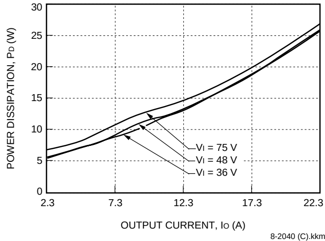
Figure 20. JFW150S6R5 Power Dissipation vs. Output Current
