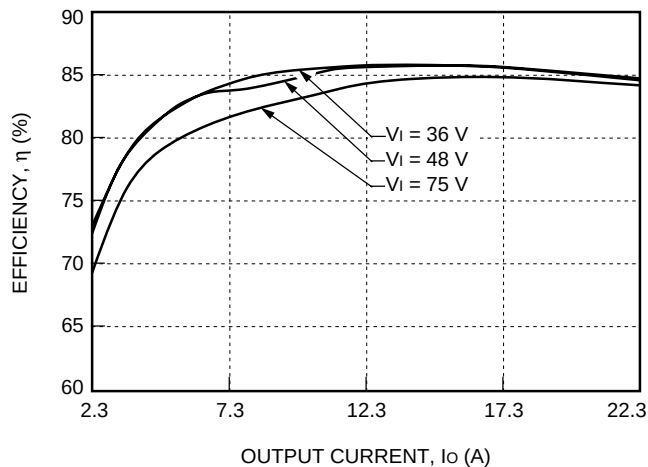
Figure 3. Typical JFW150S6R5 Converter Efficiency vs. Output Current at Room Temperature
