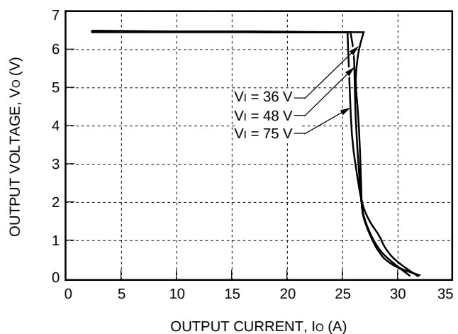
Figure 2. Typical JFW150S6R5 Output Characteristics at Room Temperature
