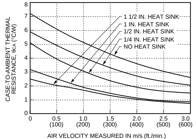
Figure 21. Case-to-Ambient Thermal Resistance Curves; Either Orientation
