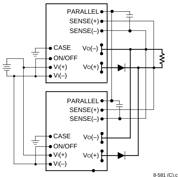
Figure 17. Wiring Configuration for Redundant Parallel Operation
