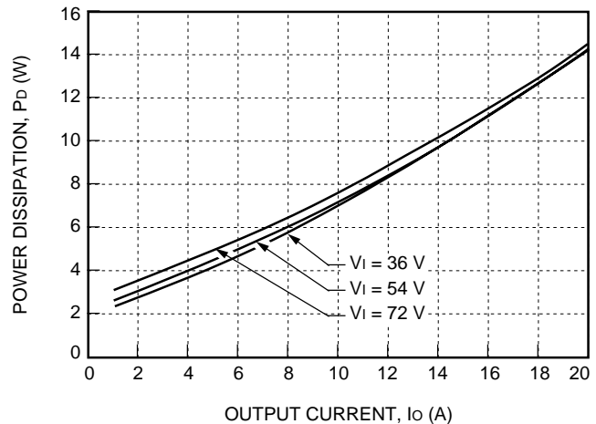
Figure 16. JW100M Power Dissipation vs. Output Current at 25 °C
