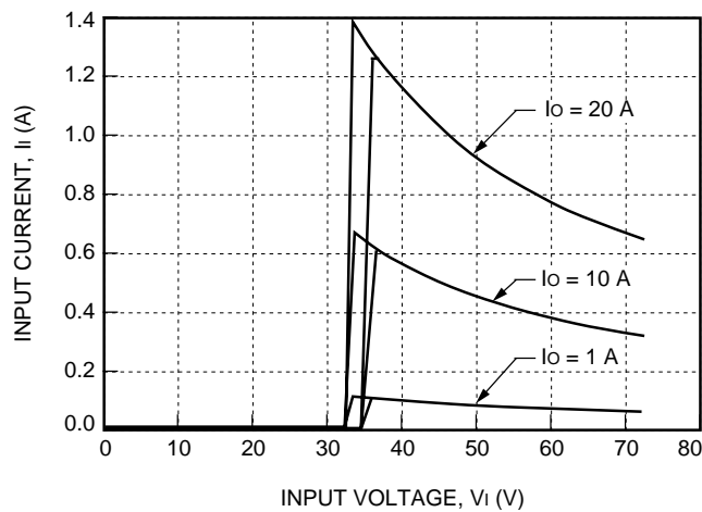
Figure 1. Typical JW100M Input Characteristics at Room Temperature
