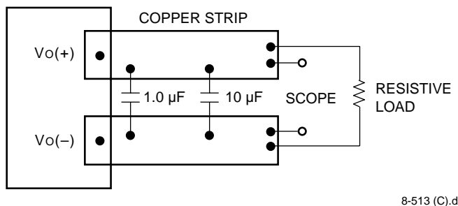
Figure 5. Input Reflected-Ripple Test Setup
