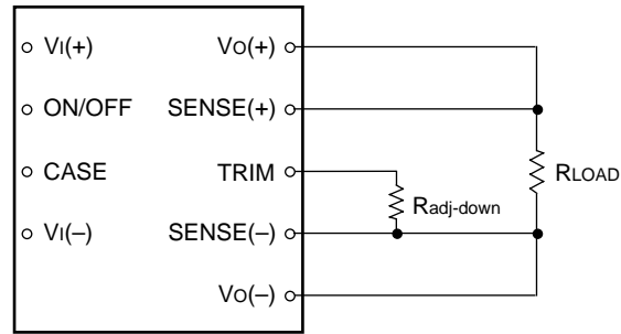
Figure 10. Circuit Configuration to Decrease Output Voltage
