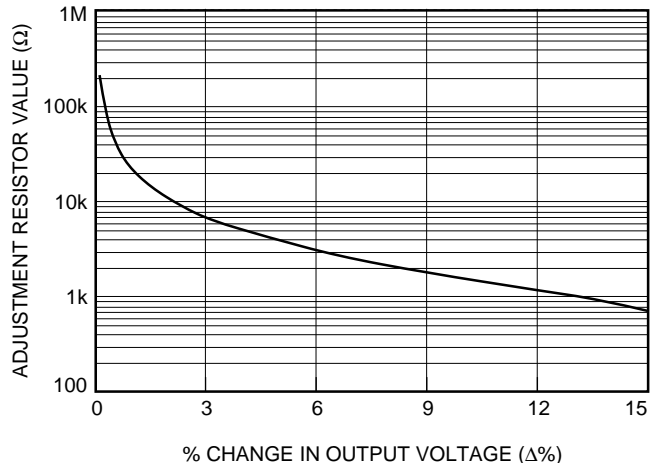
Figure 13. Resistor Selection for Increased Output Voltage
