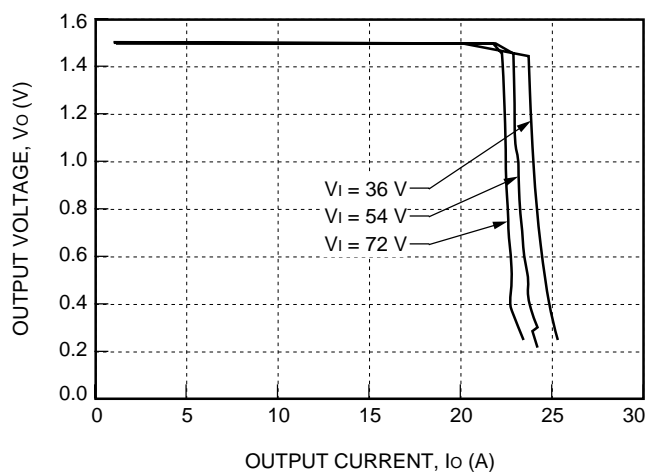
Figure 2. Typical JW100M Output Characteristics at Room Temperature
