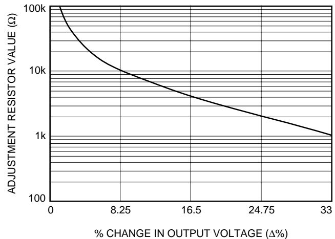
Figure 11. Resistor Selection for Decreased Output Voltage
