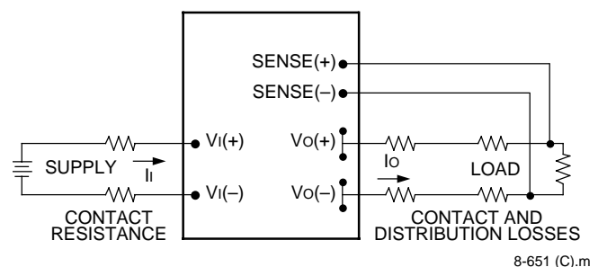
Figure 9. Effective Circuit Configuration for Single-Module Remote-Sense Operation
