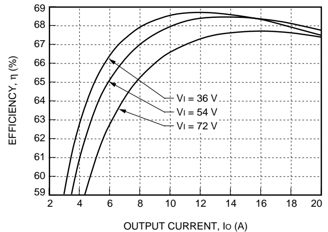
Figure 3. Typical JW100M Converter Efficiency vs. Output Current at Room Temperature
