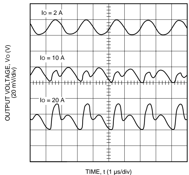
Figure 4. Typical JW100M Output Ripple Voltage at Room Temperature, 48 V Input
