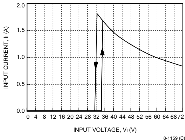
Figure 1. Typical JW050H Input Characteristics at Room Temperature
