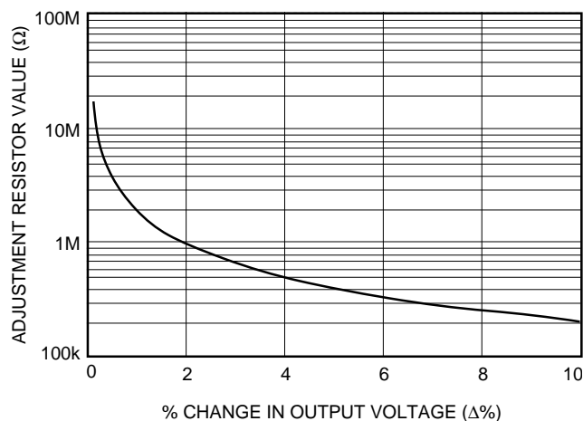
Figure 28. Resistor Selection for Increased Output Voltage
