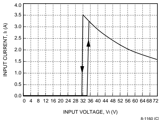
Figure 3. Typical JW100H Input Characteristics at Room Temperature
