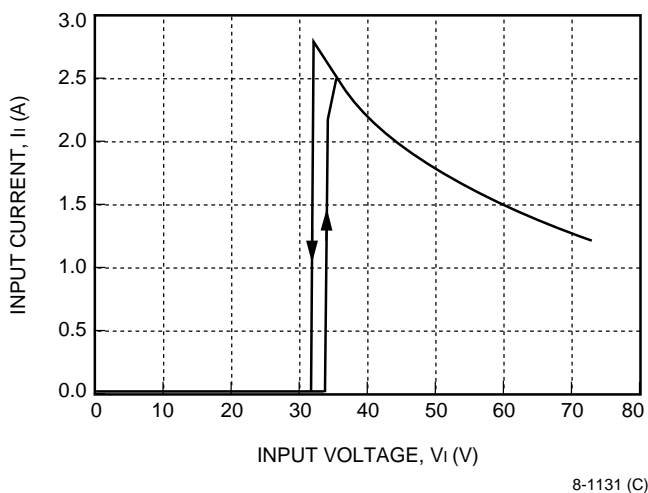
Figure 2. Typical JW075H Input Characteristics at Room Temperature
