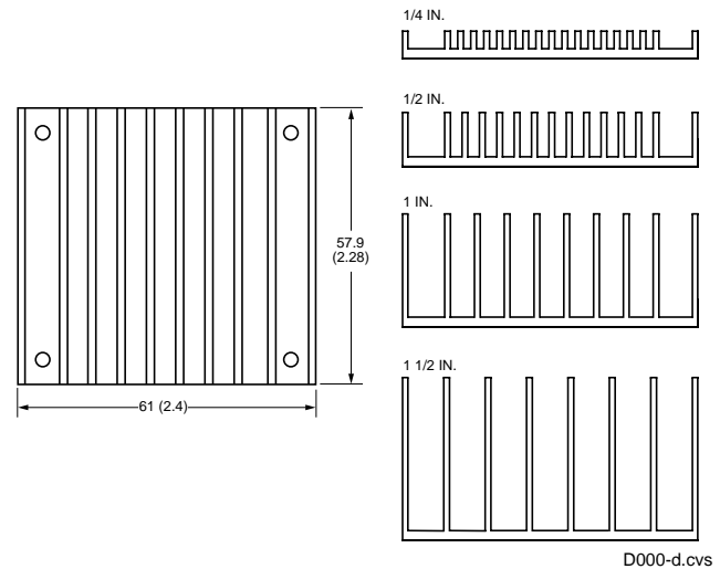
Figure 39. Transverse Heat Sink
