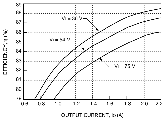
Figure 11. Typical JW050H Converter Efficiency vs. Output Current at Room Temperature
