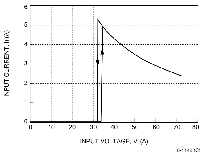
Figure 4. Typical JW150H Input Characteristics at Room Temperature
