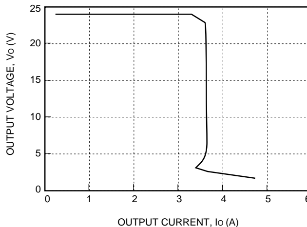
Figure 7. Typical JW075H Output Characteristics at Room Temperature
