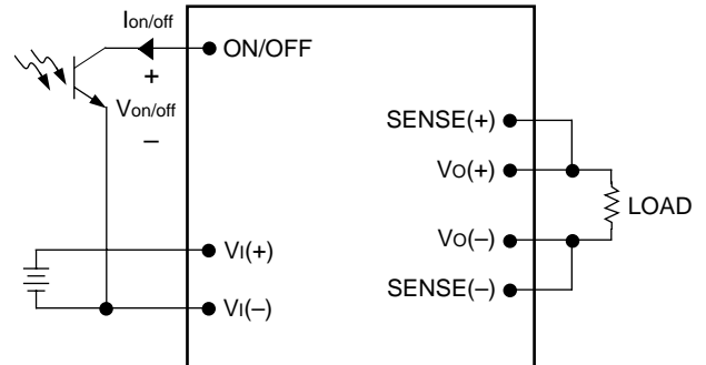
Figure 23. Remote On/Off Implementation 8-720 (C),c
