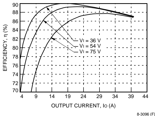
Figure 2. Typical JW040A0F Efficiency vs. Output Current at 25 °C
