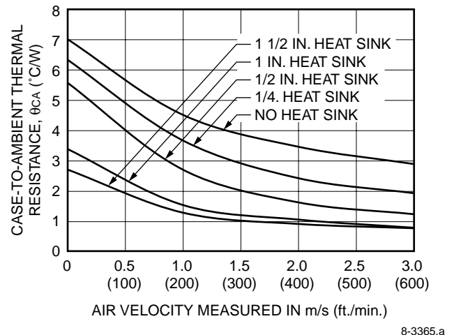
Figure 17. JW040A0F Case-to-Ambient Thermal Resistance Curves; Either Orientation
