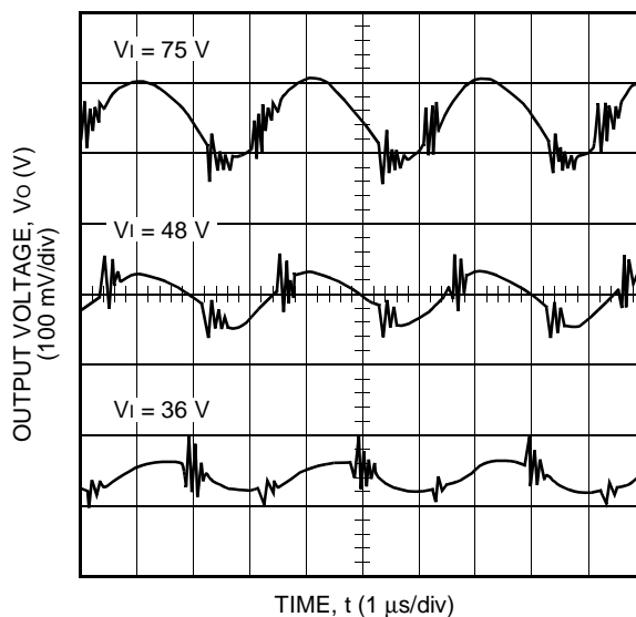
Figure 3. Typical JW040A0F Output Ripple Voltage at Room Temperature, I_o = I_{o, max}
