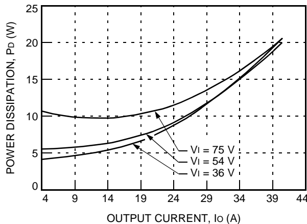
Figure 16. JW040A0F Power Dissipation vs. Output Current at 25 °C
