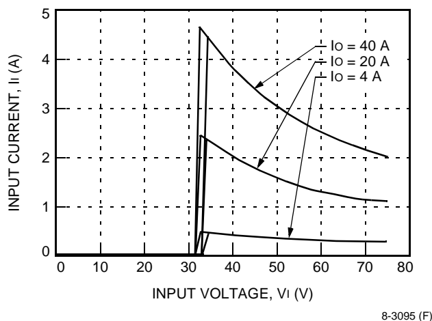
Figure 1. Typical JW040A0F Input Characteristics at 25 °C
