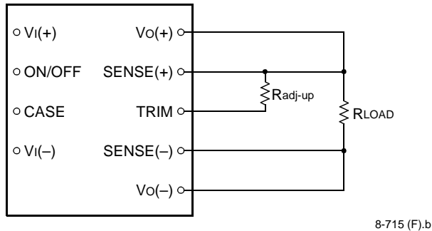
Figure 12. Circuit Configuration to Increase Output Voltage
