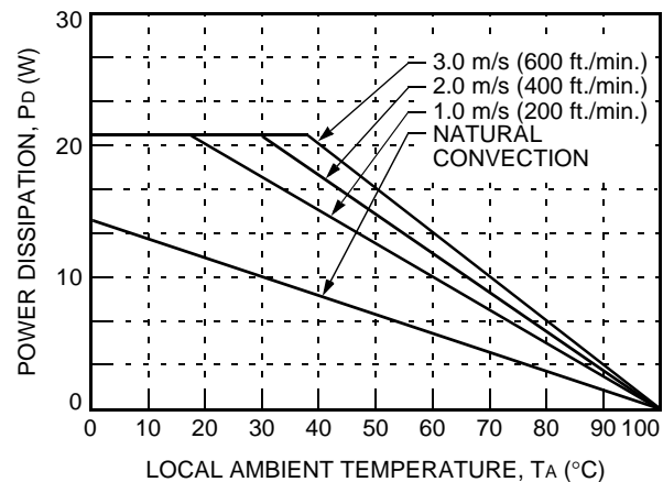
Figure 15. JW040A0F Forced Convection Power Derating with No Heat Sink; Either Orientation
