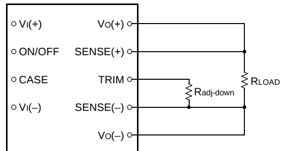
Figure 11. Circuit Configuration to Decrease Output Voltage
