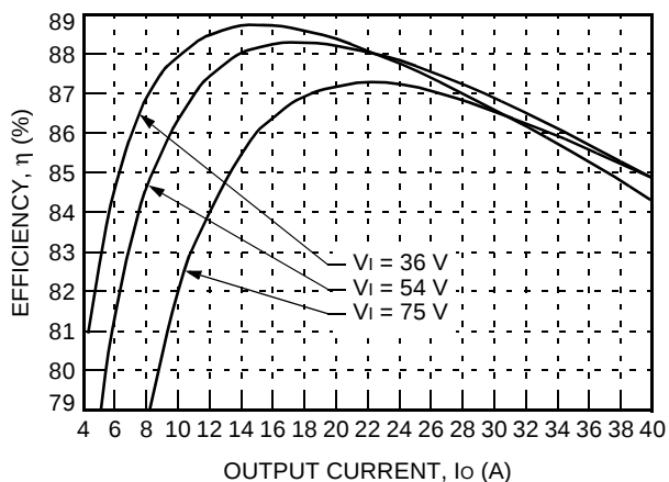
Figure 2. Typical JW040A0G Efficiency vs. Output Current at 25 °C
