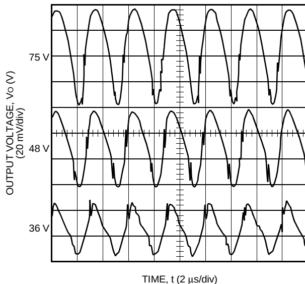
Figure 3. Typical JW040A0G Output Ripple Voltage at Room Temperature, I_o = I_{o, \max}
