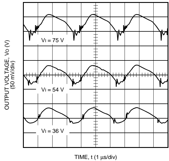
Figure 3. Typical JW040A0M Output Ripple Voltage at Room Temperature, I_o = I_{o, \max}
