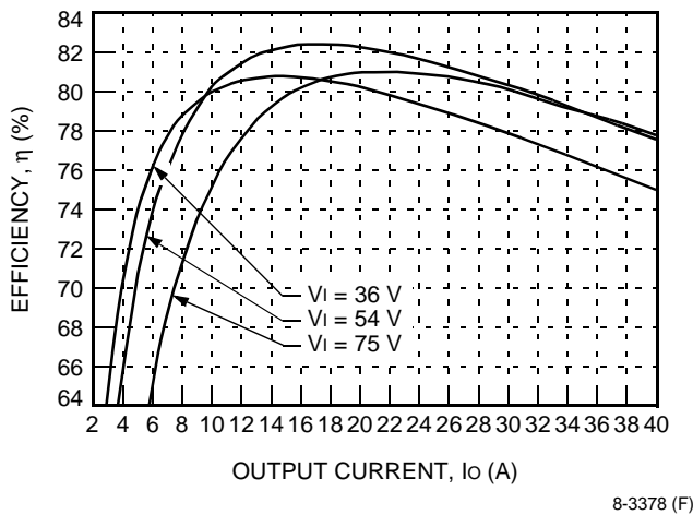
Figure 2. Typical JW040A0M Converter Efficiency vs. Output Current at Room Temperature
