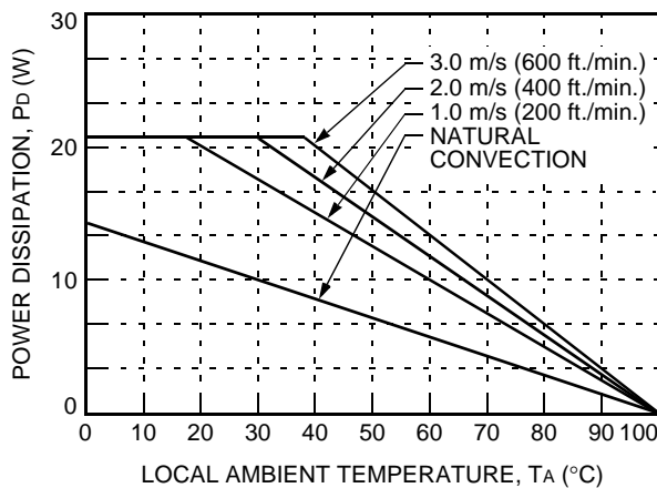
Figure 15. JW040A0M Forced Convection Power Derating with No Heat Sink; Either Orientation
