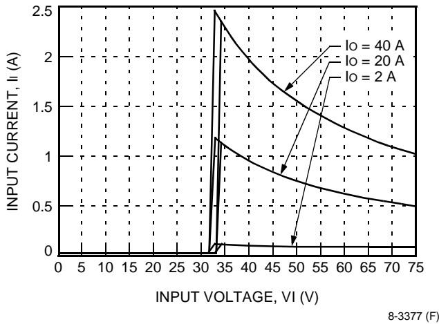
Figure 1. Typical JW040A0M Input Characteristics at Room Temperature
