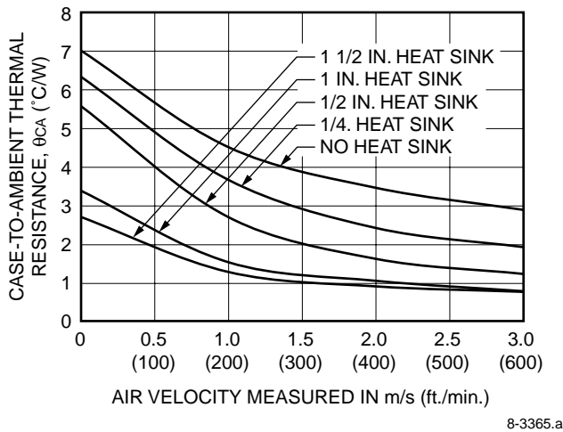
Figure 17. JW040A0M Case-to-Ambient Thermal Resistance Curves; Either Orientation
