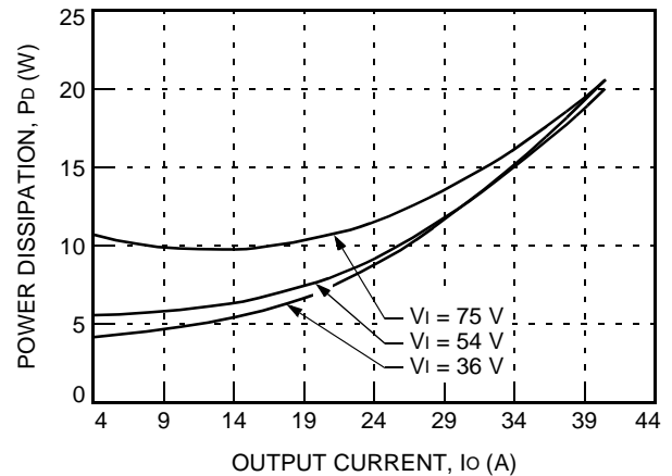
Figure 16. JW040A0M Power Dissipation vs. Output Current at 25 °C
