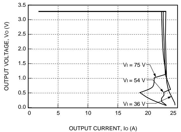
Figure 7. Typical JFW100F Output Characteristics at Room Temperature
