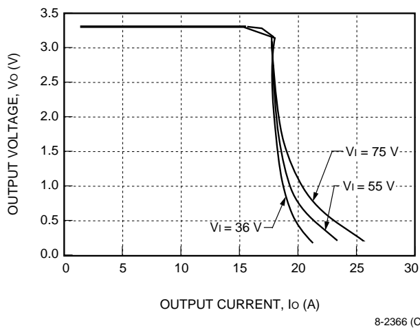
Figure 6. Typical JFW075F Output Characteristics at Room Temperature
