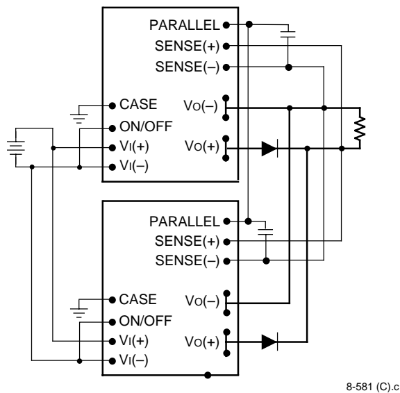
Figure 26. Wiring Configuration for Redundant Parallel Operation
