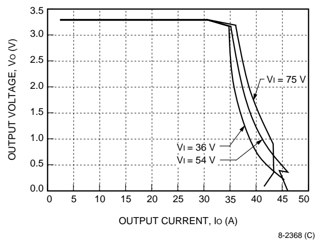
Figure 8. Typical JFW150F Output Characteristics at Room Temperature
