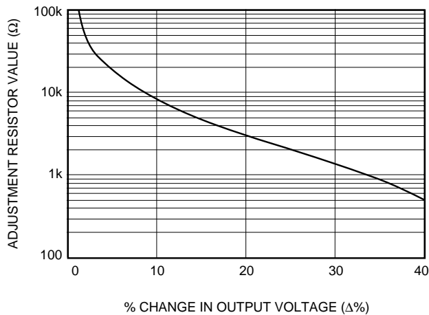
Figure 23. Resistor Selection for Decreased Output Voltage
