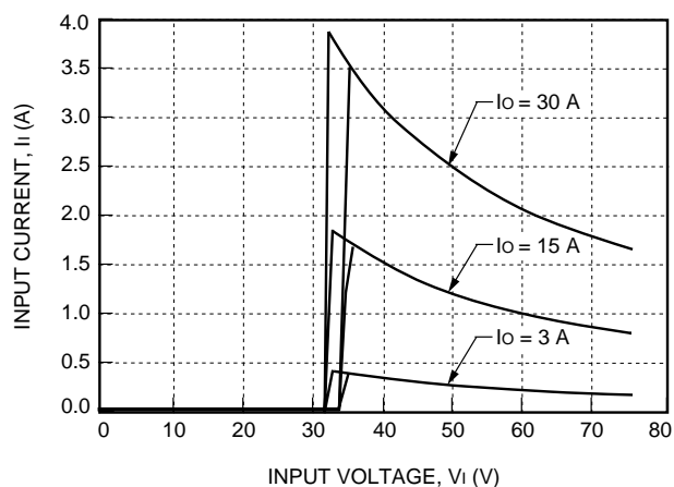
Figure 4. Typical JFW150F Input Characteristics at Room Temperature
