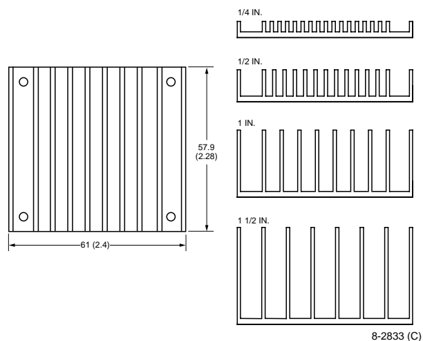
Figure 36. Transverse Heat Sink
