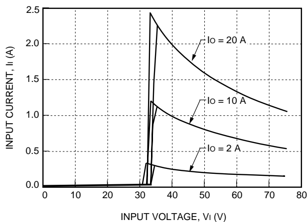
Figure 3. Typical JFW100F Input Characteristics at Room Temperature
