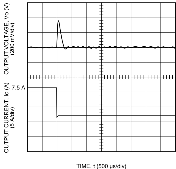
Figure 14. Typical JFW150F Transient Response to Step Decrease in Load from 50% to 25% of Full Load at Room Temperature and 54 V Input (Waveform Averaged to Eliminate Ripple Component.)
