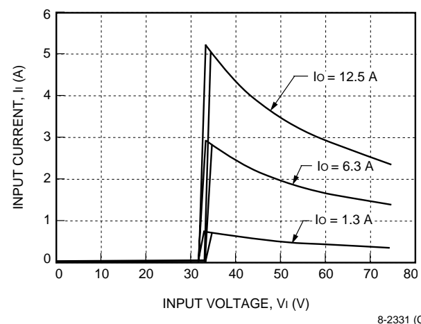
Figure 4. Typical JFW150B Input Characteristics at Room Temperature
