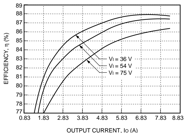
Figure 11. Typical JFW100B Converter Efficiency vs. Output Current at Room Temperature
