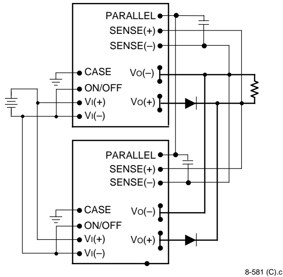
Figure 26. Wiring Configuration for Redundant Parallel Operation
