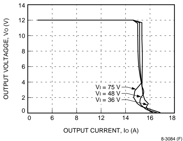
Figure 8. Typical JFW150B Output Characteristics at Room Temperature
