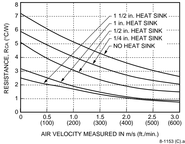
Figure 33. Case-to-Ambient Thermal Resistance Curves; Either Orientation
