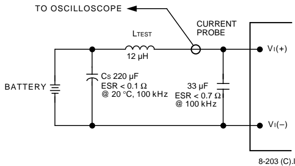
Figure 17. Input Reflected-Ripple Test Setup
