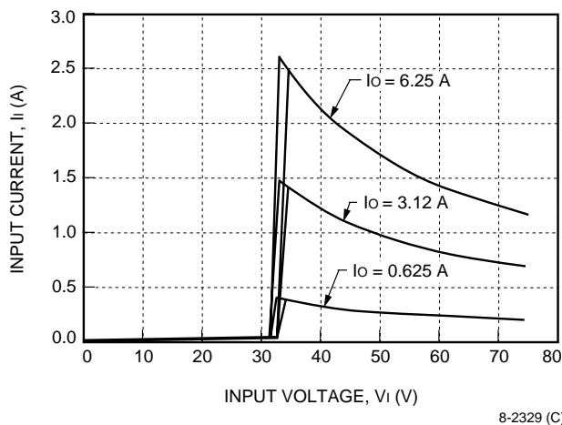
Figure 2. Typical JFW075B Input Characteristics at Room Temperature
