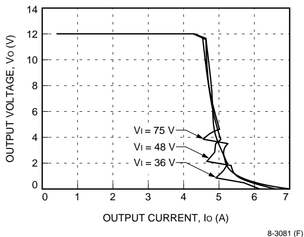
Figure 5. Typical JFW050B Output Characteristics at Room Temperature
