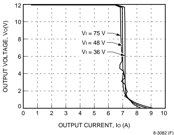
Figure 6. Typical JFW075B Output Characteristics at Room Temperature
