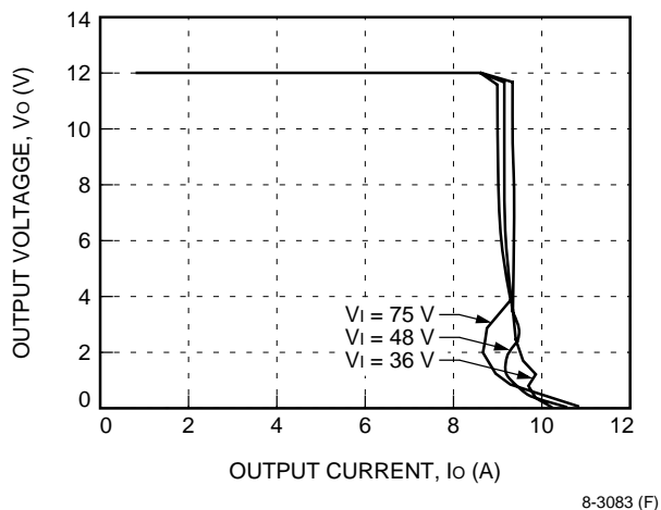
Figure 7. Typical JFW100B Output Characteristics at Room Temperature
