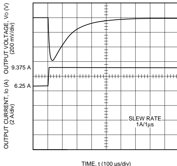
Figure 15. Typical JFW150B Transient Response to Step Increase in Load from 50% to 75% of Full Load at Room Temperature and 54 V Input (Waveform Averaged to Eliminate Ripple Component.)
