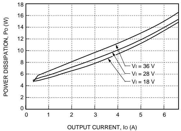
Figure 21. JFC100C Power Dissipation vs. Output Current at 25 °C
