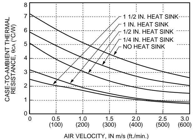
Figure 22. Case-to-Ambient Thermal Resistance Curves; Either Orientation
