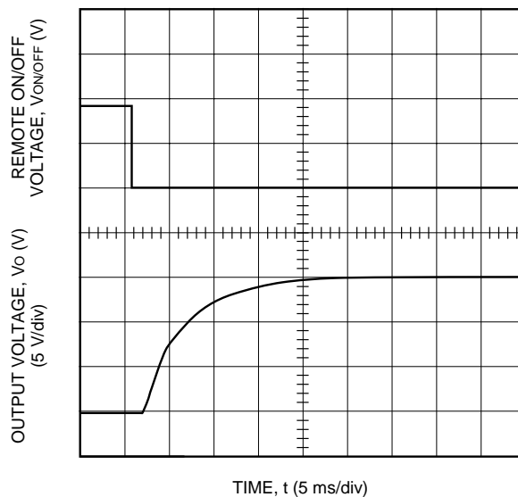
Figure 7. Typical Start-Up from Remote On/Off JFC100C1; I_o = Full Load
