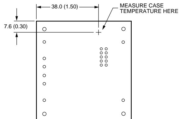
Figure 18. Case Temperature Measurement Location
