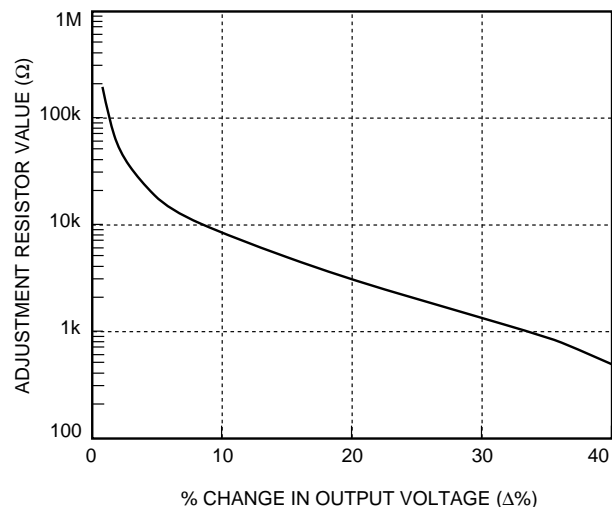
Figure 14. Resistor Selection for Decreased Output Voltage
