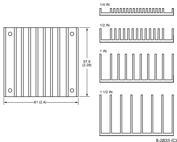
Figure 25. Transverse Heat Sink
