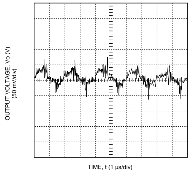
Figure 4. Typical JFC100C Output Ripple Voltage at Room Temperature, 28 V Input, Io = Full Load
