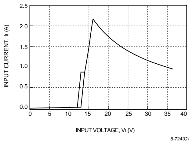
Figure 1. JC030-Series Typical Input Characteristic
