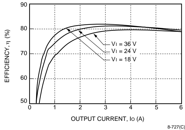
Figure 11. JC030A-M Typical Converter Efficiency vs. Output Current
