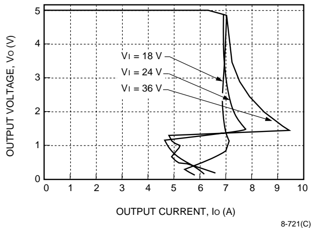
Figure 7. JC030A-M Typical Output Characteristics
