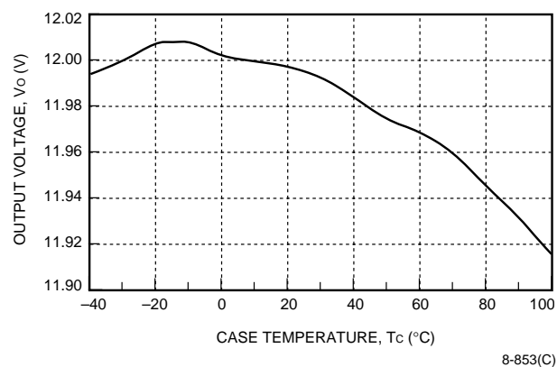
Figure 4. JC030B-M Typical Output Voltage Variation Over Ambient Temperature Range
