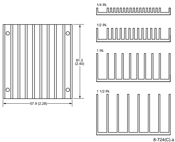
Figure 33. Longitudinal Heat Sink
