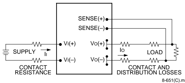
Figure 23. Effective Circuit Configuration for Single-Module Remote-Sense Operation
