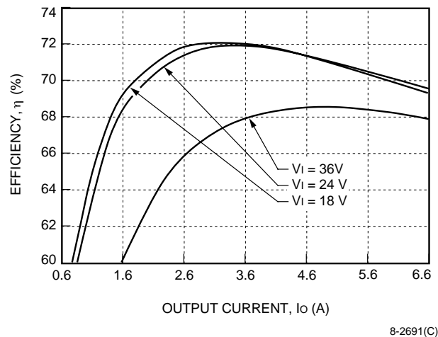
Figure 10. JC030D-M Typical Converter Efficiency vs. Output Current
