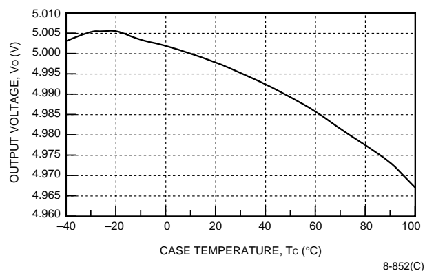
Figure 3. JC030A-M Typical Output Voltage Variation Over Ambient Temperature Range
