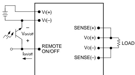
Figure 22. Remote On/Off Implementation
