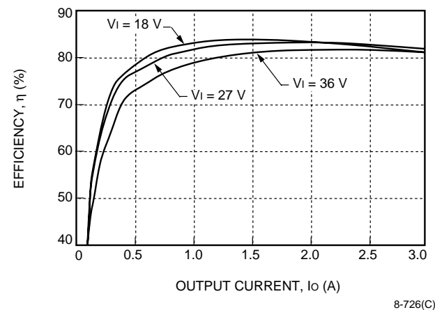
Figure 12. JC030B-M Typical Converter Efficiency vs. Output Current
