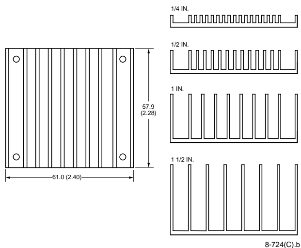
Figure 34. Transverse Heat Sink
