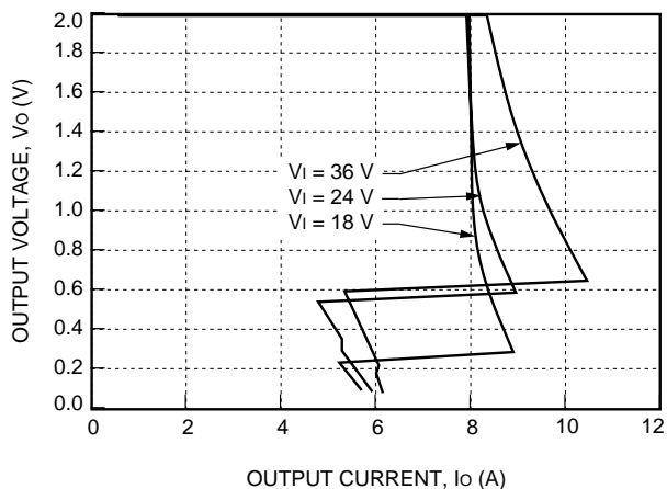
Figure 6. JC030D-M Typical Output Characteristics
