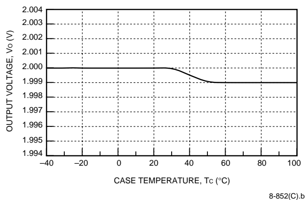
Figure 2. JC030D-M Typical Output Voltage Variation Over Ambient Temperature Range
