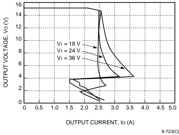
Figure 9. JC030C-M Typical Output Characteristics
