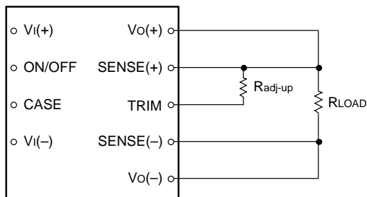
Figure 25. Circuit Configuration to Increase Output Voltage
