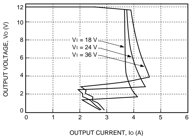
Figure 8. JC030B-M Typical Output Characteristics
