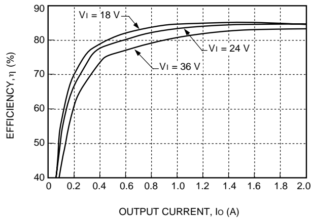
Figure 13. JC030C-M Typical Converter Efficiency vs. Output Current
