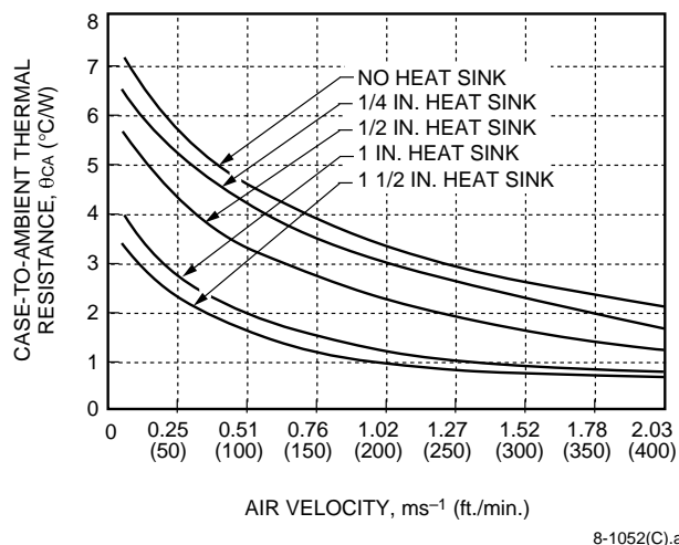
Figure 32. Case-to-Ambient Thermal Resistance vs. Air Velocity Curves; Either Orientation
