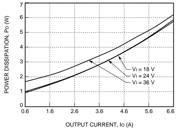
Figure 27. JC030D-M Power Dissipation vs. Output Current
