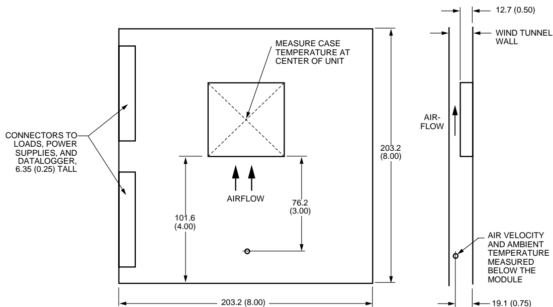
Figure 26. Thermal Test Setup
