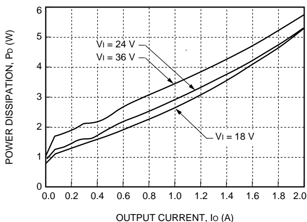
Figure 30. JC030C-M Power Dissipation vs. Output Current
