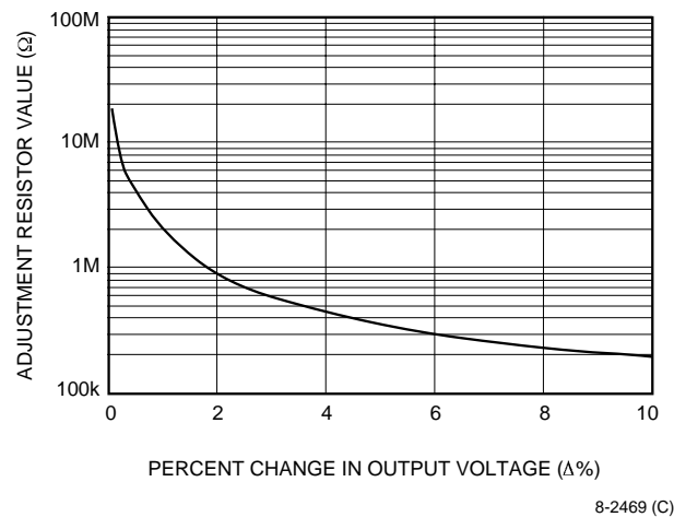
Figure 24. Resistor Selection for Increased Output Voltage
