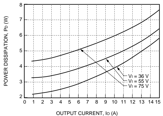
Figure 28. JAHW075F Power Dissipation vs. Output Current
