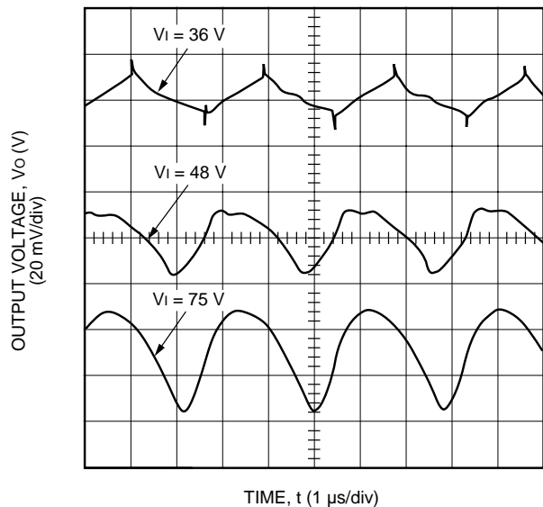
Figure 7. Typical JAHW050F and JAHW075F Output Ripple Voltage at Room Temperature and I_o = I_{o,max}
