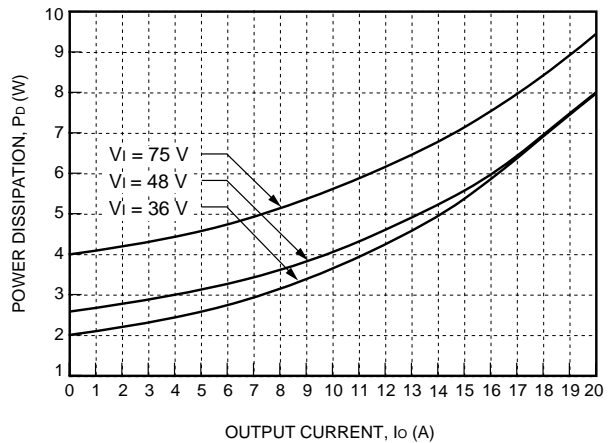
Figure 29. JAHW100F Power Dissipation vs. Output Current
