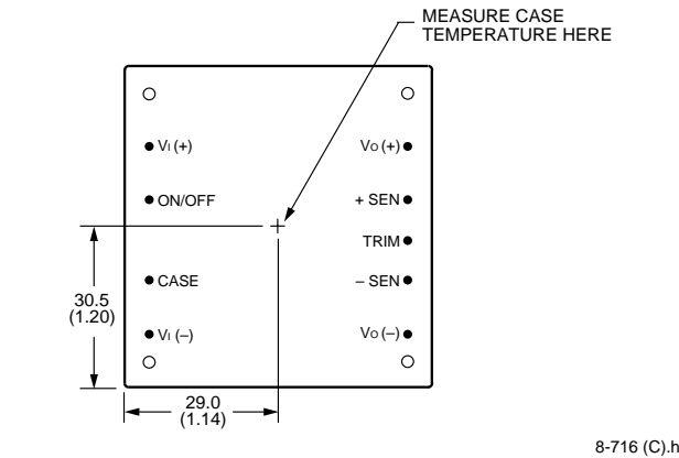
Figure 25. Case Temperature Measurement Location
