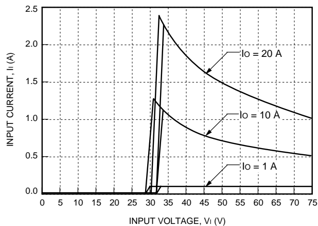
Figure 3. Typical JAHW100F Input Characteristics at Room Temperature
