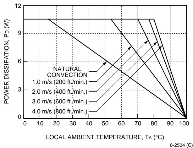
Figure 26. Forced Convection Power Derating with No Heat Sink; Either Orientation
