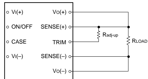
Figure 23. Circuit Configuration to Increase Output Voltage
