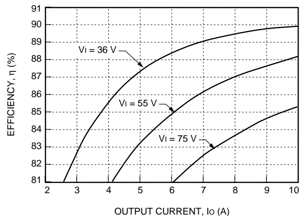
Figure 4. Typical JAHW050F Converter Efficiency vs. Output Current at Room Temperature
