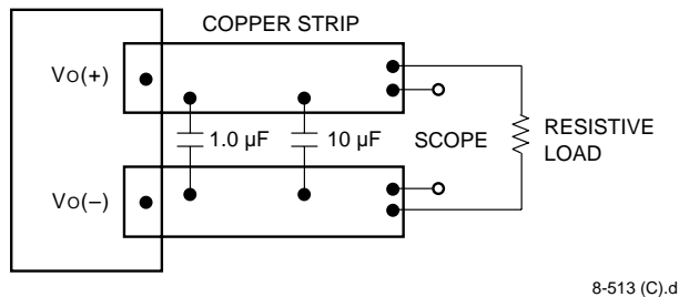
Figure 16. Input Reflected-Ripple Test Setup
