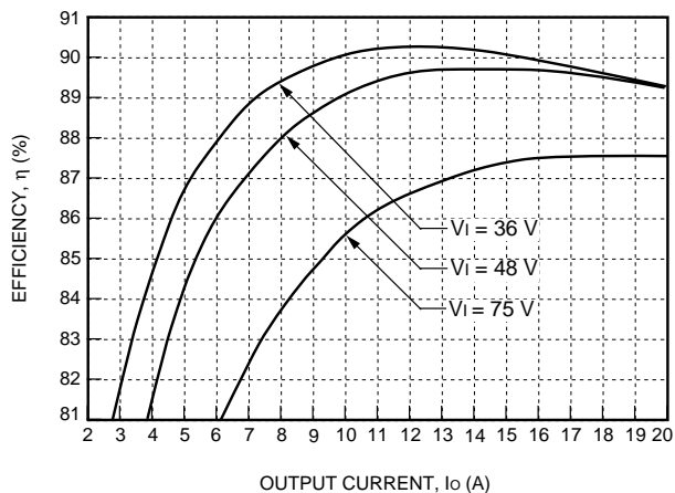
Figure 6. Typical JAHW100F Converter Efficiency vs. Output Current at Room Temperature
