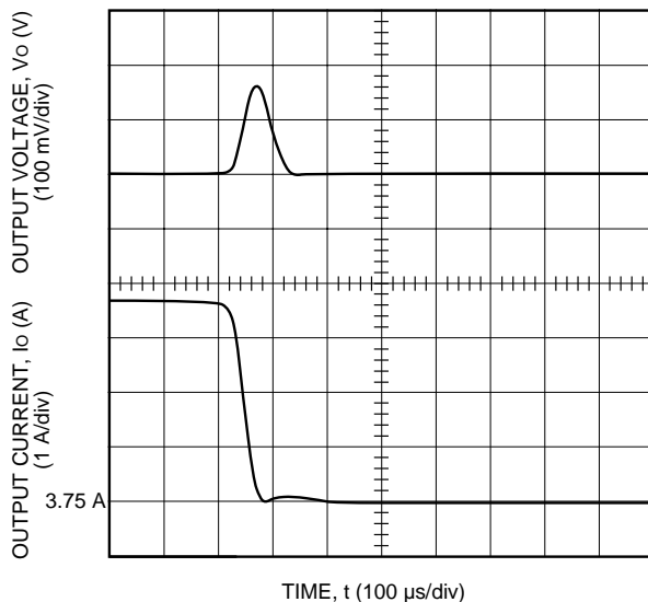
Figure 9. Typical JAHW050F Transient Response to Step Decrease in Load from 50% to 25% of Full Load at Room Temperature and 48 Vdc Input (Waveform Averaged to Eliminate Ripple Component.)
