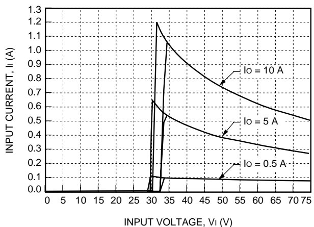
Figure 1. Typical JAHW050F Input Characteristics at Room Temperature
