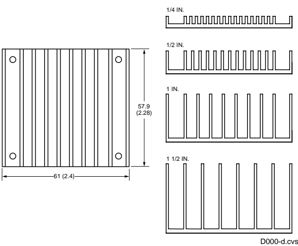
Figure 33. Transverse Heat Sink
