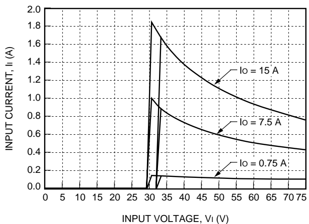
Figure 2. Typical JAHW075F Input Characteristics at Room Temperature
