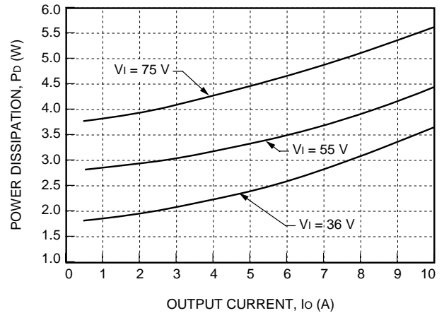
Figure 27. JAHW050F Power Dissipation vs. Output Current
