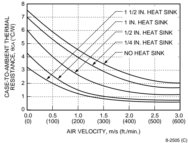
Figure 30. Case-to-Ambient Thermal Resistance Curves; Either Orientation
