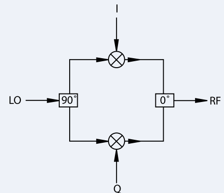
I&Q modulation block diagram
