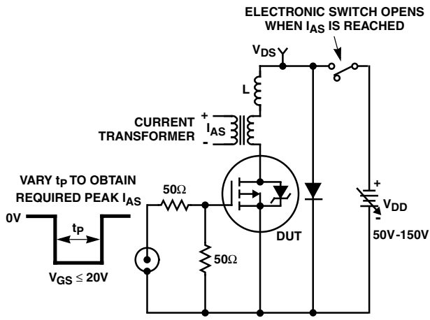
FIGURE 9. UNCLAMPED ENERGY TEST CIRCUIT
