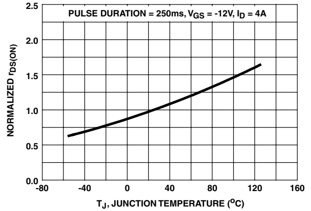
FIGURE 6. NORMALIZED r_{DS(ON)} vs JUNCTION TEMPERATURE
