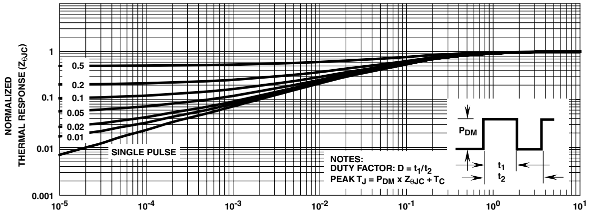
FIGURE 7. NORMALIZED MAXIMUM TRANSIENT THERMAL RESPONSE
