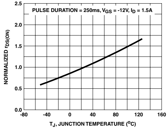
FIGURE 6. NORMALIZED r_{DS(ON)} vs JUNCTION TEMPERATURE
