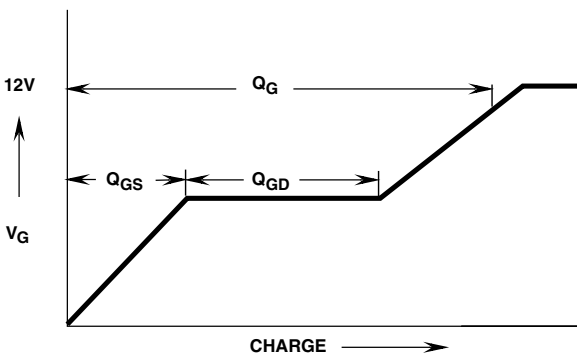
FIGURE 5. BASIC GATE CHARGE WAVEFORM
