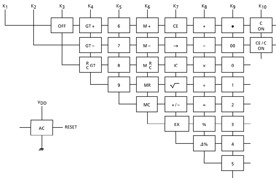
Touch Key
