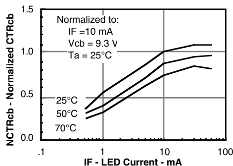
Figure 8. Normalized \text{CTR}_{cb} versus LED current and temperature
