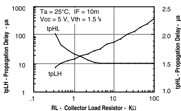
Figure 14. Propagation delay versus collector load resistor
