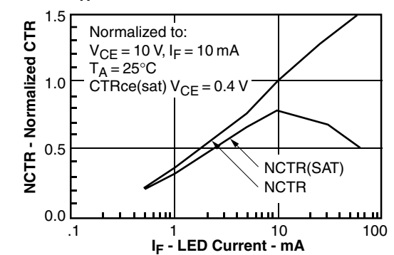
Figure 2. Normalized non-saturated and saturated CTR at T_A=25^\circ\text{C} versus LED current
