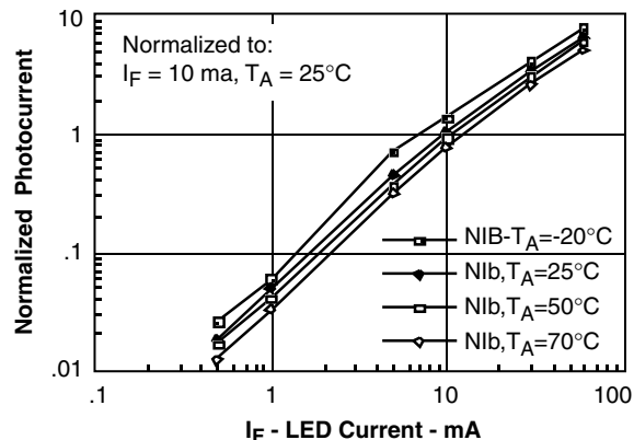
Figure 10. Normalized photocurrent versus I_F and temperature
