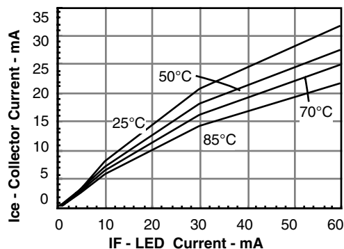
Figure 6. Collector-emitter current versus temperature and LED current
