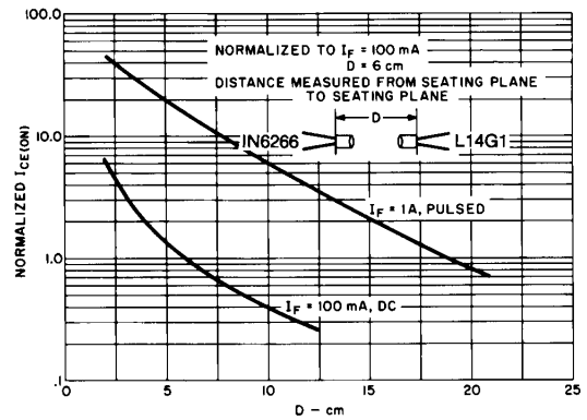
Fig. 3. I_c vs. Distance IRED/Phototransistor Pair
