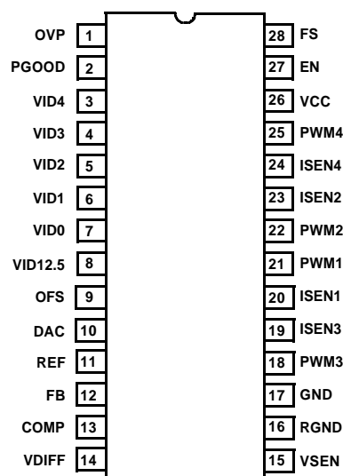
28-PIN SOIC TOP VIEW
