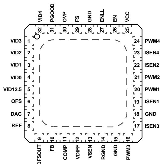
32-LEAD QFN TOP VIEW
