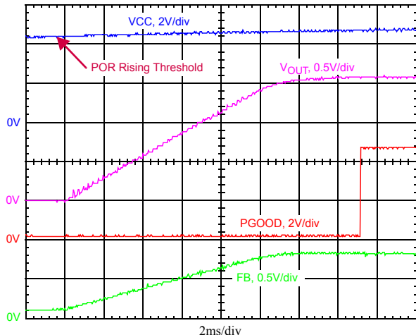
FIGURE 3. SOFT-START WAVEFORMS
