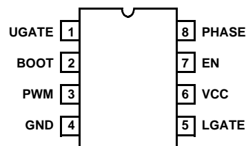
ISL6605 8 LEAD (SOIC) TOP VIEW
