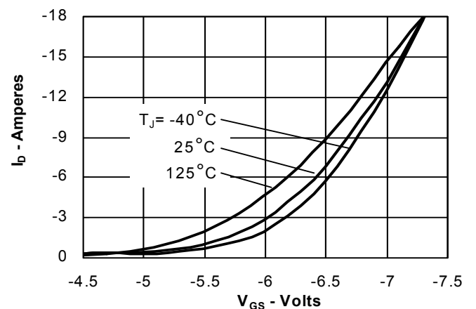
Fig. 6. Input Admittance
