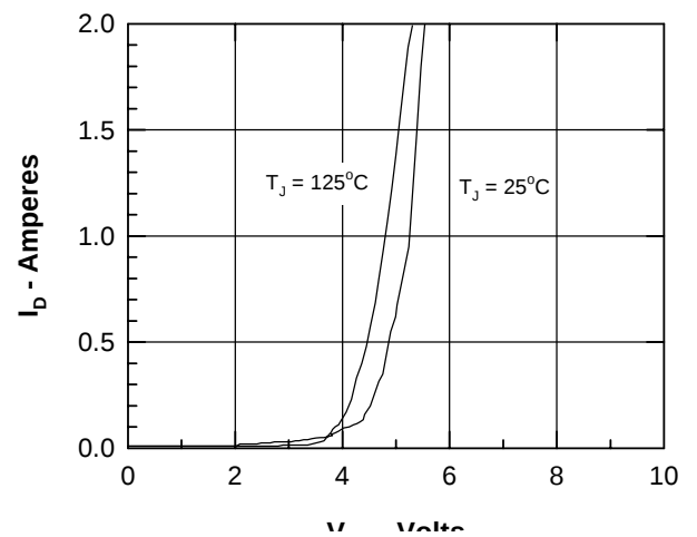
Figure 6. Admittance Curves
