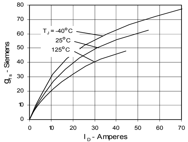
Fig. 8. Transconductance
