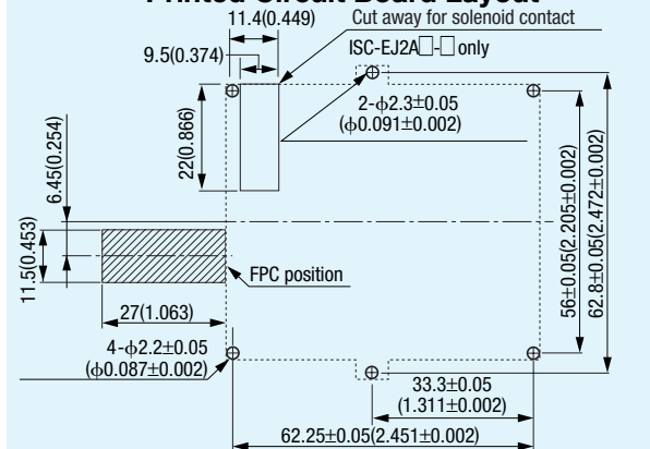
Printed Circuit Board Layout
