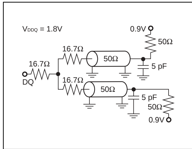
Figure 2 ( V_{DDQ} = 1.8V )
