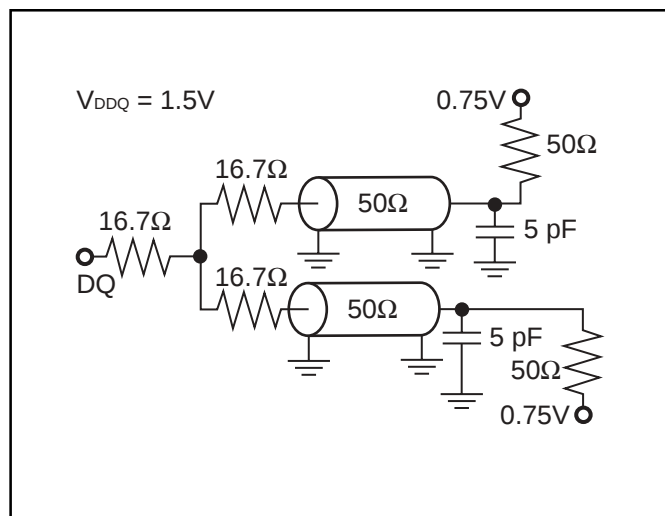
Figure 1 ( V_{DDQ} = 1.5V )
