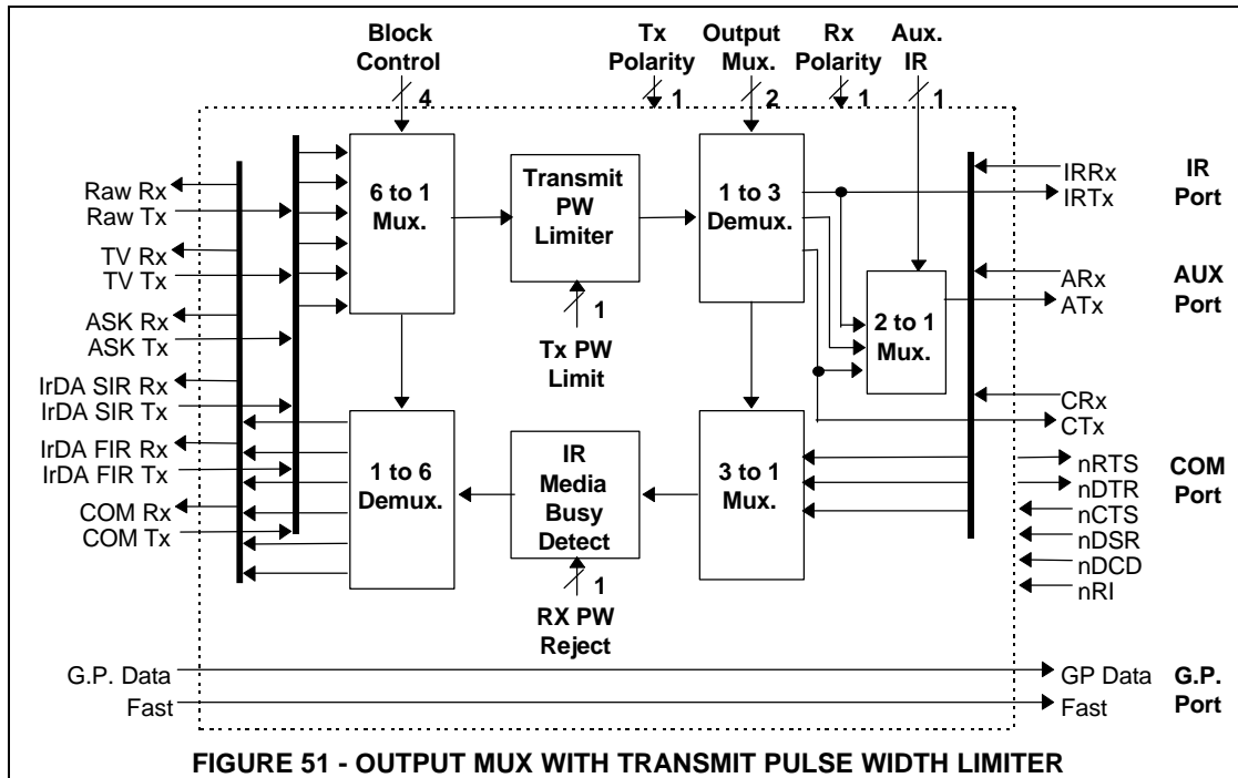
FIGURE 51 - OUTPUT MUX WITH TRANSMIT PULSE WIDTH LIMITER
