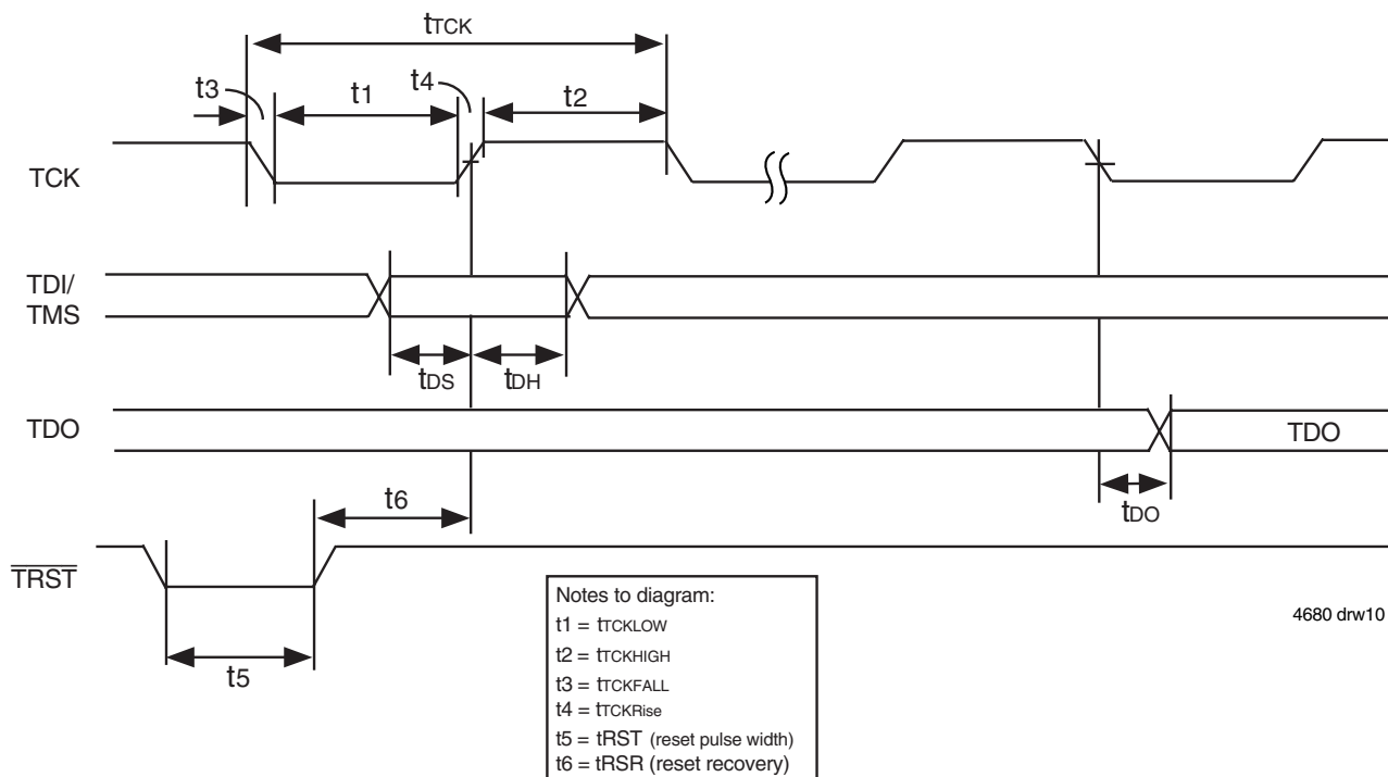
Figure 5. Standard JTAG Timing
