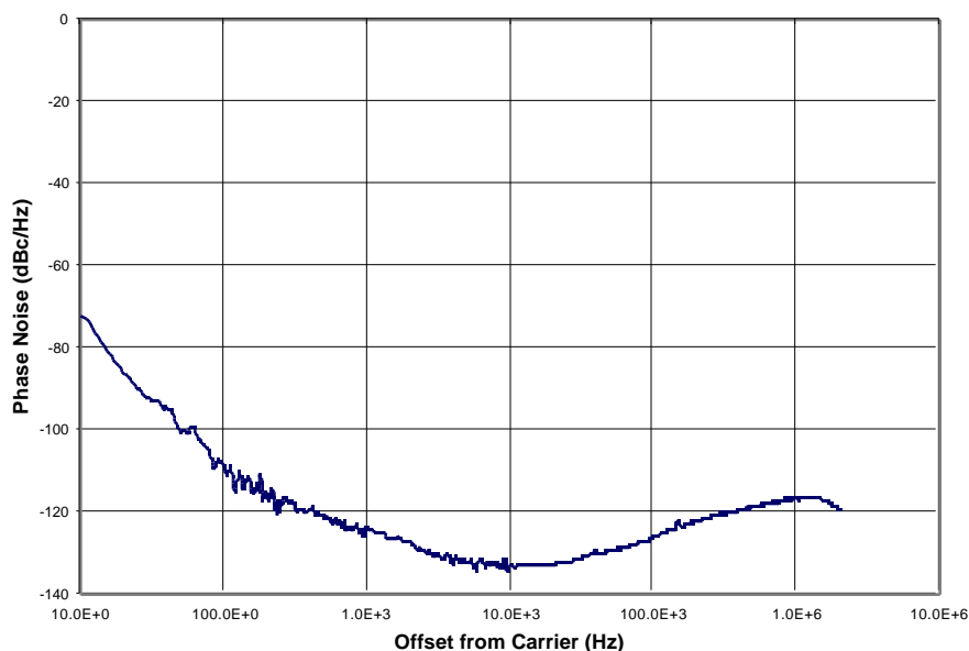
Figure 1. Phase Noise of ICS601-01 at 125 MHz out, 25 MHz crystal input.
