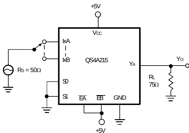
NOTE: 1. Off-isolation = 20 \log |V_o/V_s|
