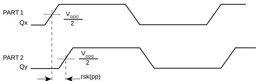
PART-TO-PART SKEW
