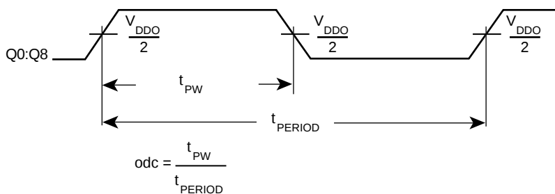
t_{PW} & t_{PERIOD}
