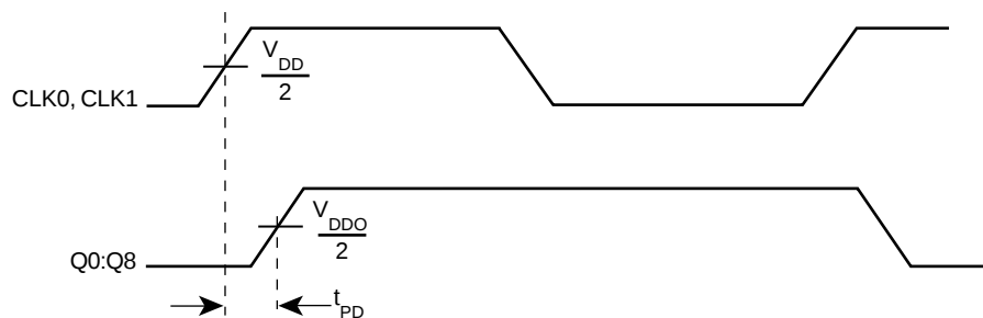
PROPAGATION DELAY
