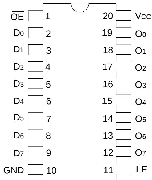
QSOP TOP VIEW
