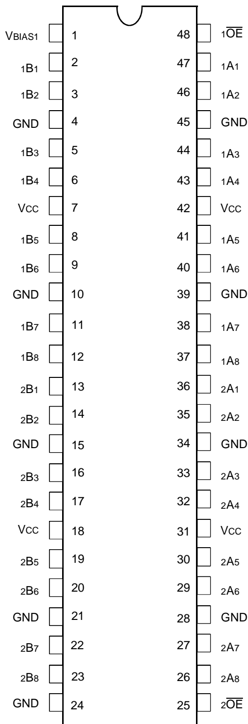
TSSOP/ TVSOP TOP VIEW
