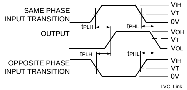
Propagation Delay
