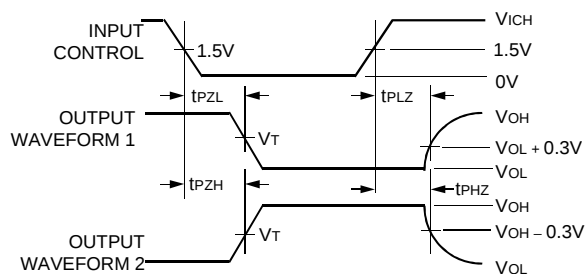
Voltage Waveforms Enable and Disable Times (OAx) ( V_{IH} = 5V for V_{CC} = 5V , 3V for V_{CC} = 3.3V ) ( V_T = V_{CC}/2 for V_{CC} = 5V , 1.5V for V_{CC} = 3.3V )
