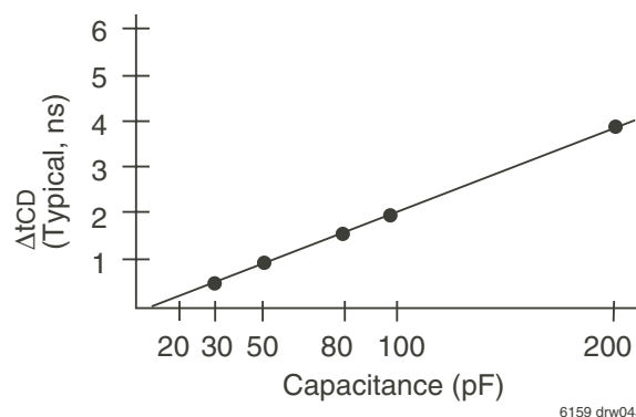
Figure 2b. Lumped Capacitive Load, Typical Derating
