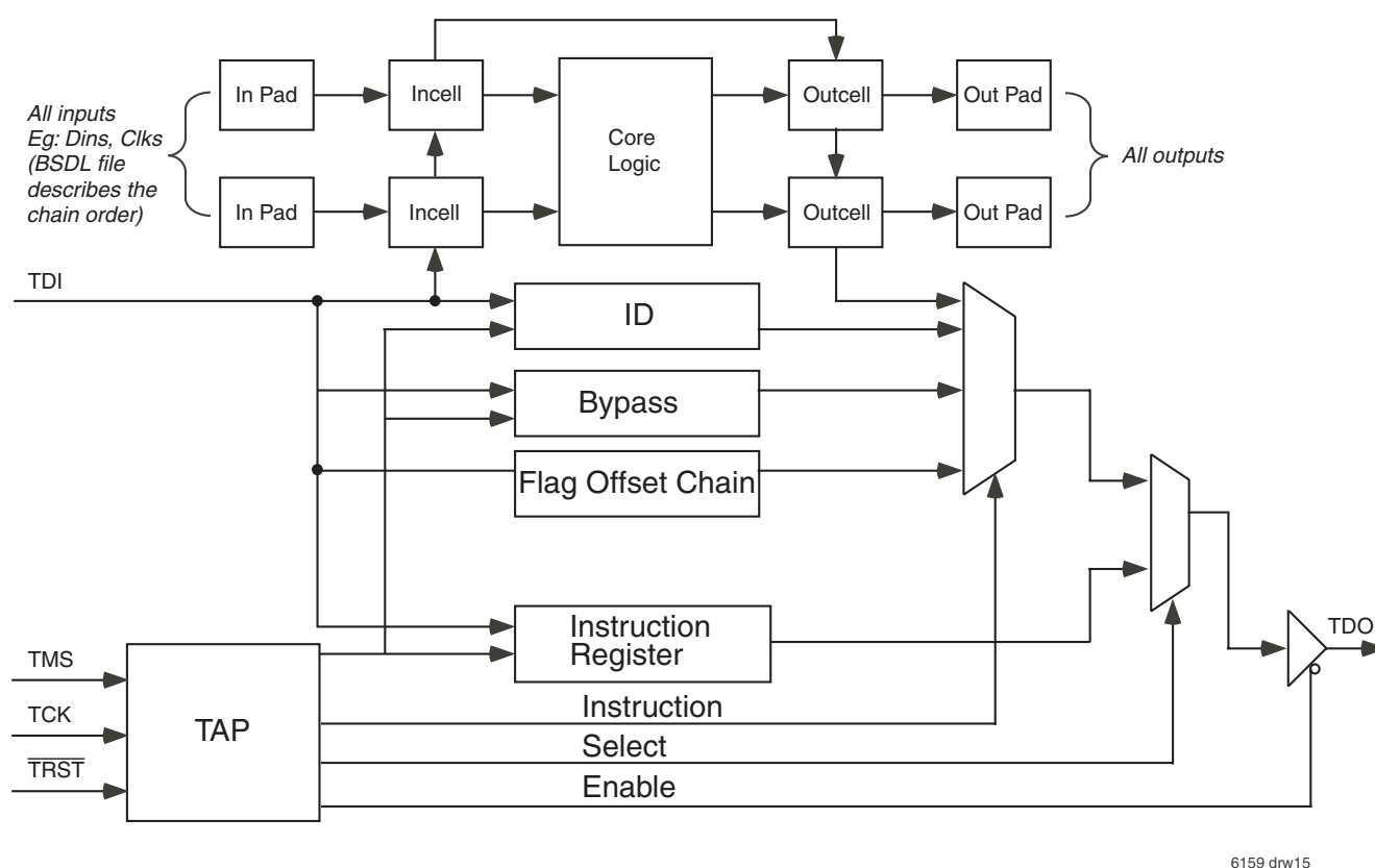
Figure 8. JTAG Architecture
