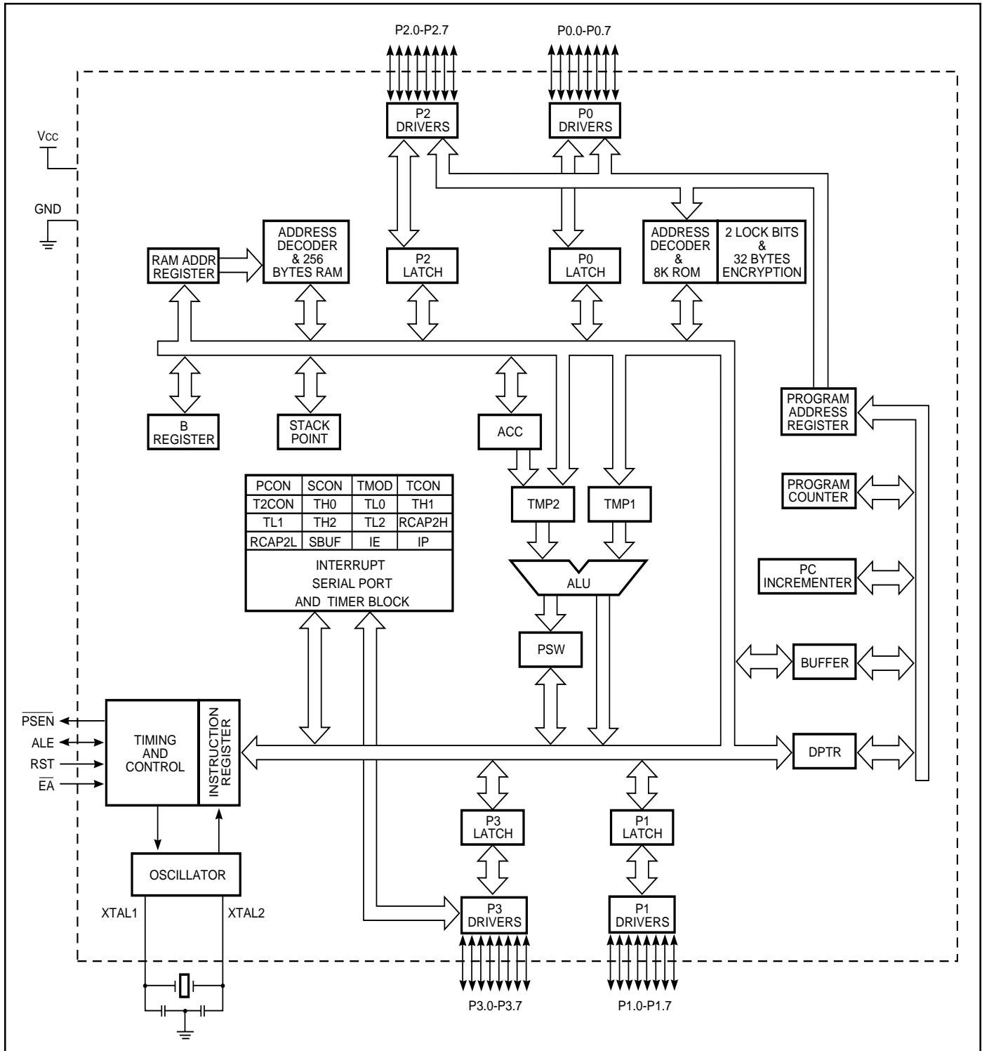
Figure 4. IS80C52/32 Block Diagram
