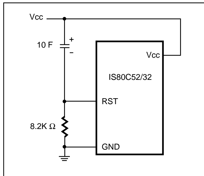
Figure 21. Power-On Reset Circuit
