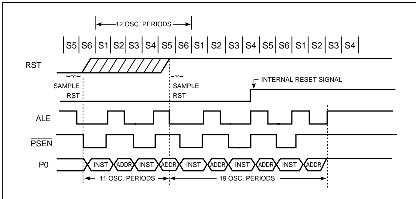
Figure 22. Reset Timing
