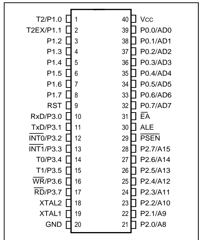
Figure 1. IS80C52/32 Pin Configuration: 40-pin DIP
