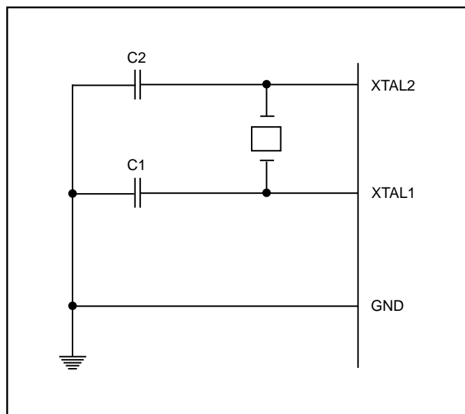
Figure 24. Oscillator Connections
