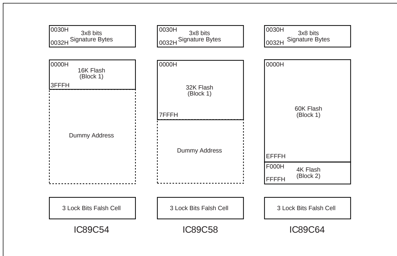
Figure 5. The Flash Architecture of IC89C54/58/64
