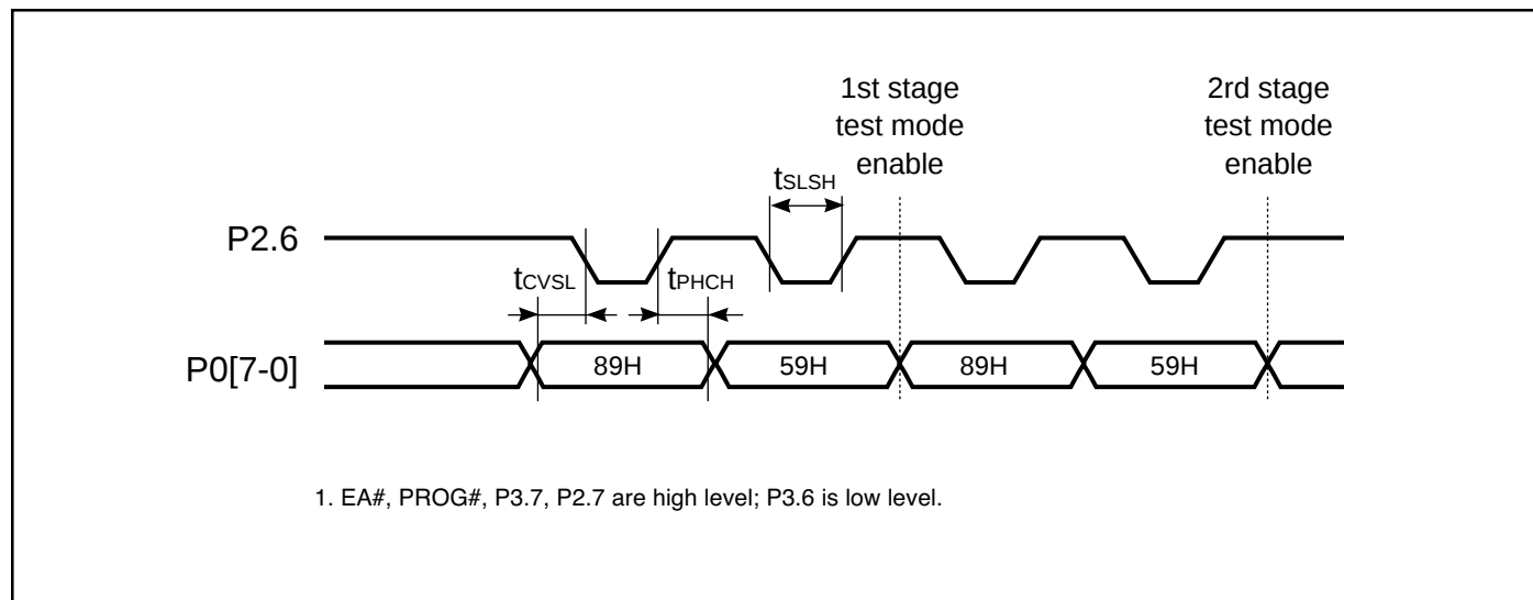
Figure 18. Test Mode Entering Timing
