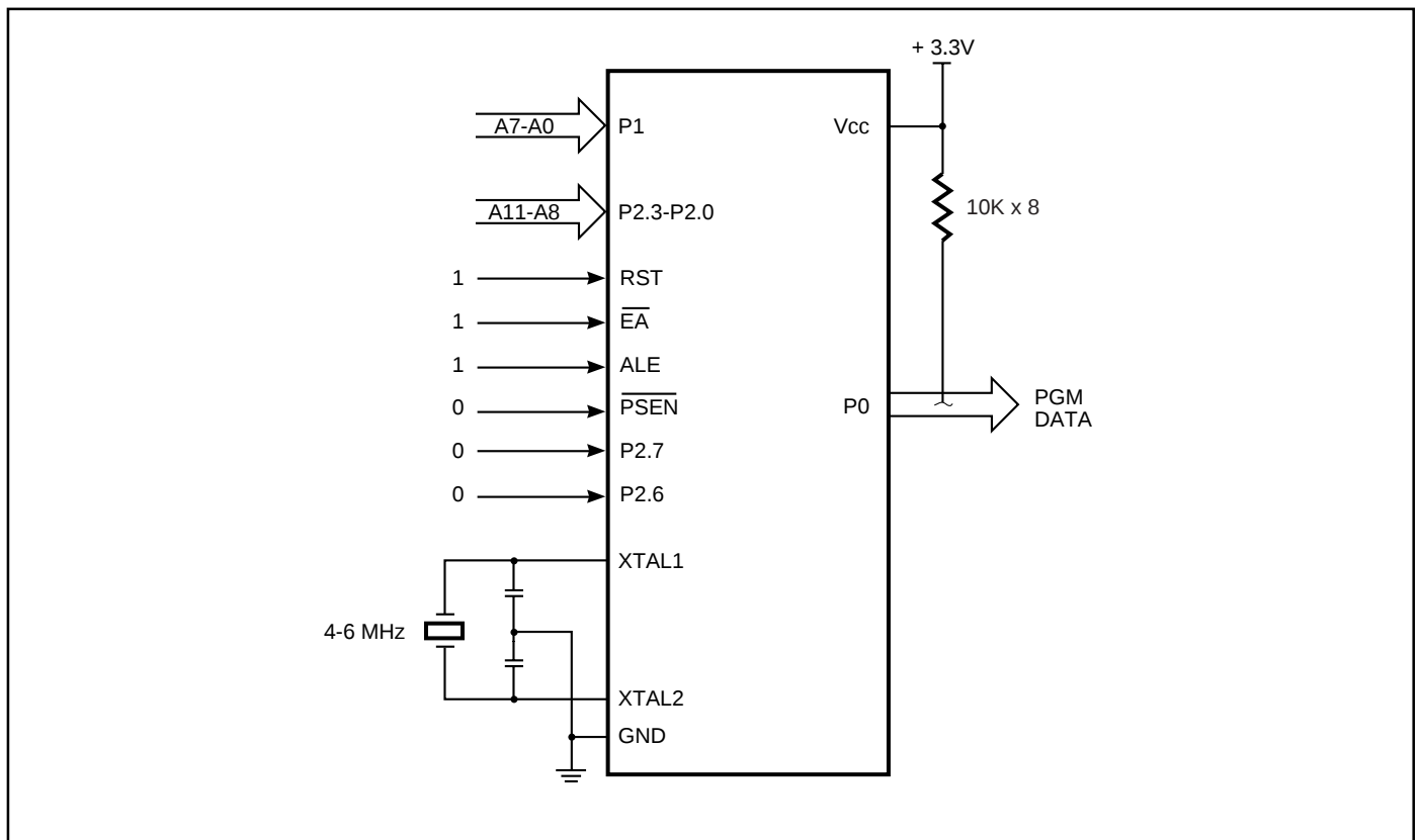
Figure 10. ROM Verification
