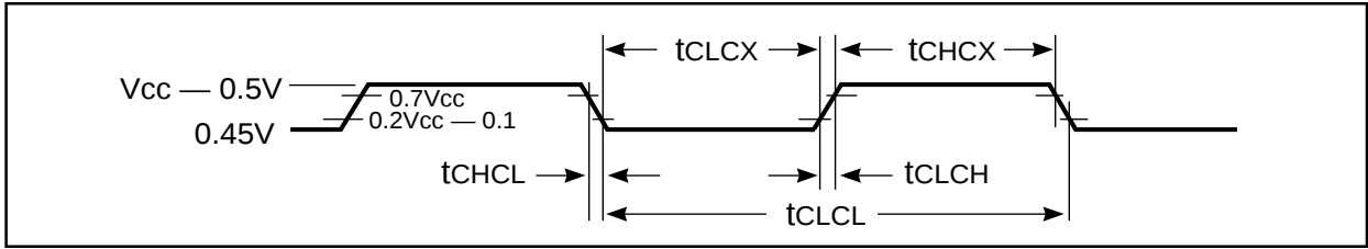
Figure 14. Clock Signal Waveform for Icc Tests in Active and Idle Modes. ( t_{CLCH} = t_{CHCL} = 5 \text{ ns} )
