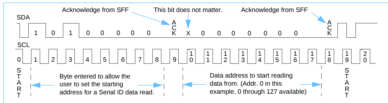
Serial ID Figure 3 Read Data Sequence Timing
