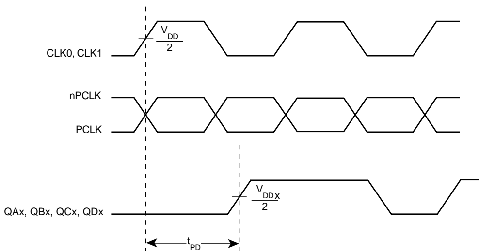
PROPAGATION DELAY
