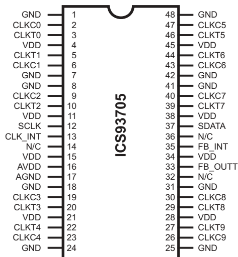
48-Pin SSOP
