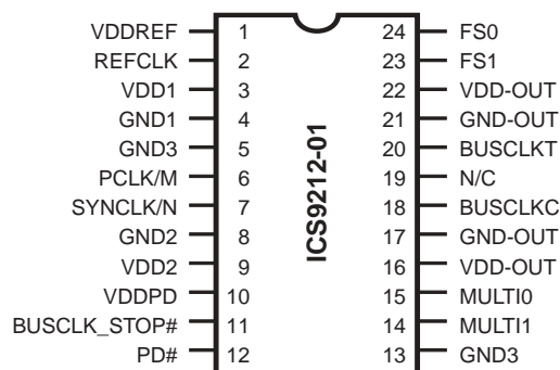
24-Pin 150 Mil SSOP
